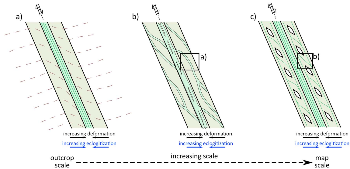
Figure 8. Schematic illustration of the general shear zone geometries on different scales: (a) outcrop scale showing the general setup of strong deformation and eclogitization in the central part (darker green) and the transitional (light green) degree of eclogitization and deformation outward into the unaltered granulite (light red). Red and green lines show the granulite- and eclogite-facies foliations, respectively. (b) Intermediate scale showing how the single small-scale shear zones (a) form shear zone networks. Here there is typically a central part with many and wider shear zones and a transitional zone with fewer and less pronounced shear zones (light green) until only the unaltered granulite remains. (c) Typical schematic illustration of the map-scale shear zones with the completely eclogitized and strongly deformed shear zone in the center bounded by eclogite breccia.
