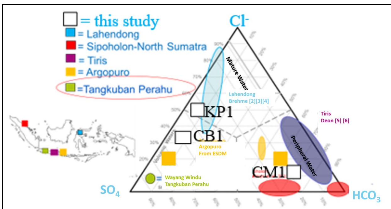
Figure 6. Ternary diagram of the major anions \text{Cl}^- , \text{SO}_4^{2-} , \text{HCO}_3^- . Data from the literature show significant differences in the geochemistry from different fields and are included for comparison.
