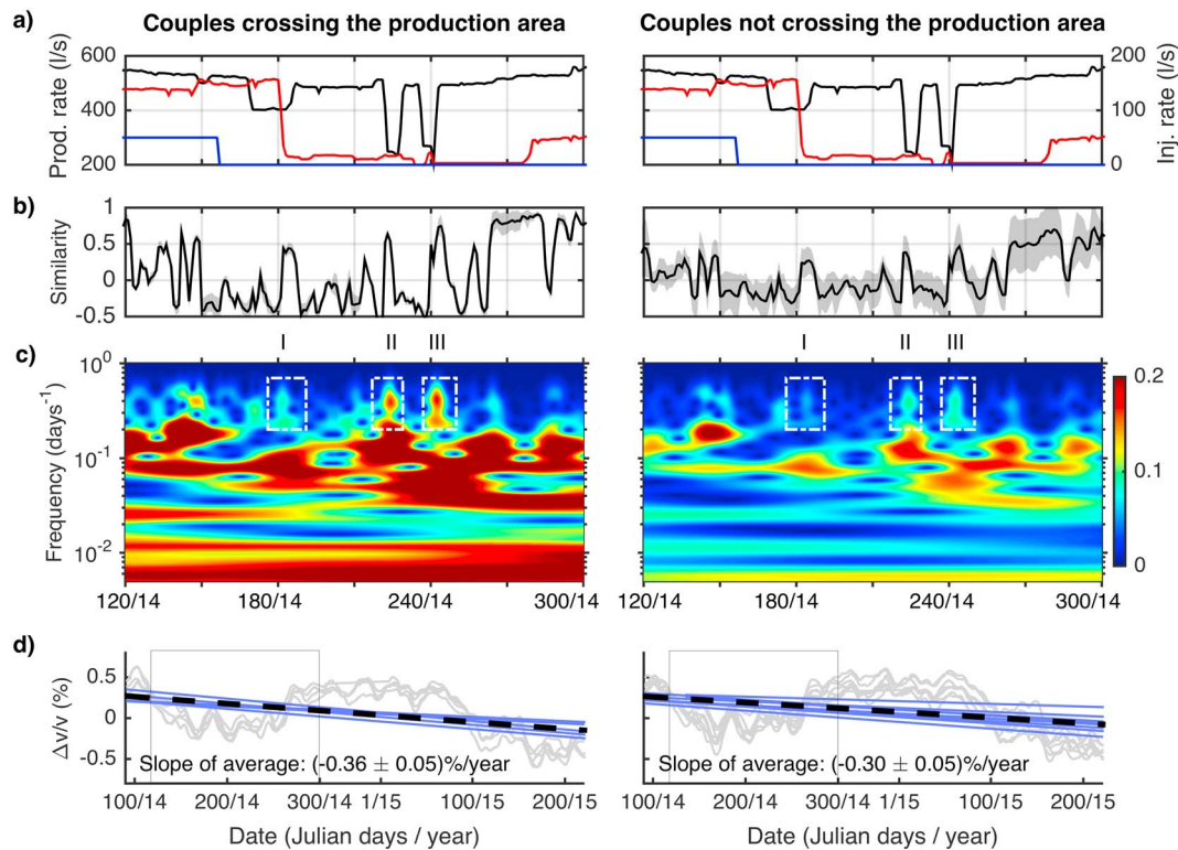
Figure 3. (a) Production and injection rate of Reykjanes Geothermal System. The colors are the same as on Figure 2a. (b) Average of similarity values of station couples that cross (left) and do not cross (right) the production area at 6-s lag time. Standard deviation is shown as gray shading. (c) Time-frequency amplitude spectra of the above similarity curves. The white boxes highlight the fluctuations I, II, and III. (d) Velocity variations measured using the generalized MWCS formulation for \beta = 10^4 (gray lines) of autocorrelations for the 1.5 years of study. The blue lines represent their linear regressions of every curve, and the dashed black line, the linear regression of the velocity variation average of the station group. The gray box marks the period of time of the upper panels.
