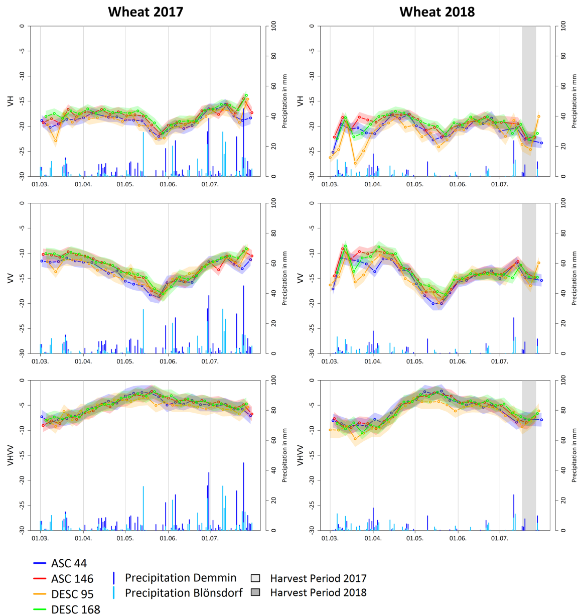
Figure 5. Temporal profiles of backscatter parameters VV, VH and VH/VV of wheat fields in 2017 (left) and 2018 (right). Standard deviations are depicted as polygons around lines. Blue bars represent daily precipitation sums for the test sites Demmin (dark blue) and Blönsdorf (light blue).
