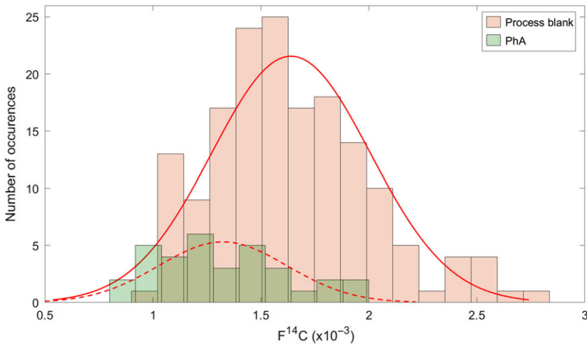
Figure 2 Distributions of F^{14}\text{C} for 166 process blanks (Kauri and Brown coal wood, red) and 33 combustible blanks (PhA, green) measured at ETH-Zürich over 2 years are fitted with normal distributions (red lines).
