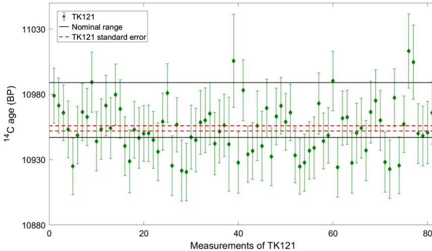
Figure 3 ^{14}\text{C} age for 81 reference samples (TK121, green) measured at ETH-Zürich with their mean value ( 1\text{-}\sigma limits, red lines) and the nominal value (black, see Methods section).
