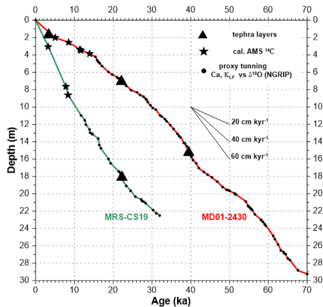
Figure 4. Age–depth model for cores MD01–2430 and MRS-CS19 from the Sea of Marmara created using calibrated AMS ^{14}\text{C} ages (stars) and multiparameter tuning to the NGRIP ice core record (Svensson et al. 2006, 2008) and published ages of tephras, Avellino (AV) (Hammer et al. 1987; Sevink et al. 2011), Cape Riva (Y-2) (Pichler & Friedrich 1976; Eriksen et al. 1990; Druitt et al. 1999; Roeser et al. 2012; Fabbro et al. 2013) and Campanian Ignimbrite tephra (CI/Y-5) (Fisher et al. 1993; De Vivo et al. 2001; Giaccio et al. 2017). Radiocarbon dates and tephra ages were used as initial tie points for the age models. XRF Ca and \kappa_{\text{LF}} features (solid dots) were then correlated between those age tie points to the NGRIP \delta^{18}\text{O} record.
