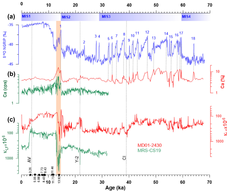
Figure 3. Magnetic susceptibility ( \kappa_{LF} ) and Ca ( \mu -XRF-count per second; cps) for cores MRS-CS19 and MD01–2430 from the Sea of Marmara tuned to \delta^{18}O data from the NGRIP over the last 70 ka. (a) Greenland NGRIP ice core \delta^{18}O record (GIC05 time scale) (Svensson et al. 2006, 2008) and MIS boundaries (blue bars). Numbers in the NGRIP plot indicate Dansgaard-Oeschger warming events (Dansgaard et al. 1993; Svensson et al. 2006, 2008; Rasmussen et al. 2006; Wolff et al. 2010); (b) XRF Ca records from cores MD01–2430 (Çağatay et al. 2015) and MRS-CS19 (this study); (c) magnetic susceptibility data after simultaneous tuning to the \delta^{18}O record in (a). Dashed vertical lines mark the stratigraphic positions of tephra layers AV (Avellino), Y-2 (Cape Riva), CI (Campanian Ignimbrite, Y-5) and correlation point between Ca and NGRIP record. Diamond and circles show radiocarbon ages of MRS-CS19 and MD01–2430, respectively. The orange vertical bar marks the lacustrine-marine transition zone.
