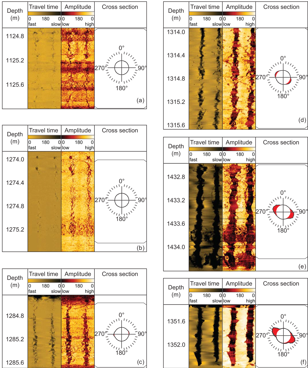
Figure 10. Snapshots from different development stages of borehole breakouts. (a) The first stage in the borehole breakout formation starts by initiation of vertical structures with almost similar appearance as drilling-induced fractures. The many micro fractures propagate and merge and hence chips of the rock begin to spall off the wall (c and d). The cross sections in (a) and (b) are still almost circular, although in travel time and amplitude images, the incipient breakouts are already visible. In time, more portion of rocks spall off the borehole wall, and the breakouts get more developed and ultimately show the typical almost oval “circle-with-ears” shape in the cross section (e and f).
