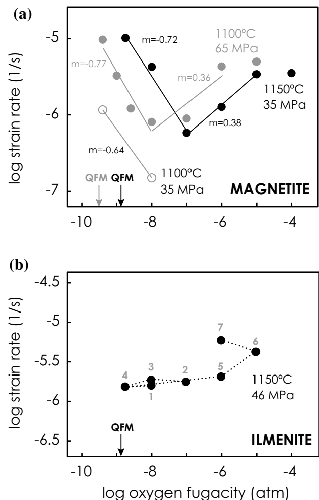
Fig. 8 Dependence of oxide single-crystal creep rates on oxygen fugacity for a magnetite compressed along \langle 111 \rangle at various temperatures and compressive stresses, and b ilmenite compressed normal to \langle 0001 \rangle . Grey and black arrows indicate the oxygen fugacity of the QFM buffer at 1100 and 1150°C, respectively. Solid lines in a are fits to parts of the data set representing regions of negative and positive creep dependence on f_{O_2} . Numbers next to each data point in b indicate the order of the creep steps
