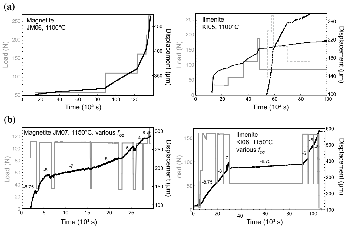
Fig. 2 Representative mechanical data from creep experiments on a magnetite and b ilmenite single crystals. Dashed lines for experiment KI05 represent creep segments for the repeated temperature step at 1100 °C. Creep segments in (b) are labeled with oxygen fugacities in log atm units
