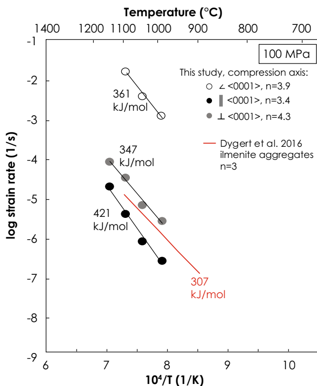
Fig. 7 Arrhenius plot of ilmenite single-crystal creep data from this study normalized to a stress of 100 MPa. Activation energies are indicated for each experiment. The dislocation creep flow law for synthetic ilmenite aggregates from Dygert et al. (2016) is shown for comparison
