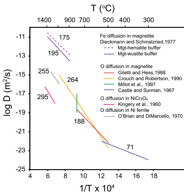
Fig. 10 Arrhenius plot of reported Fe and O diffusivities in magnetite and experimental data for O diffusion in other spinel-structured oxides. Labels for each data set represent activation energies in kJ/mol
