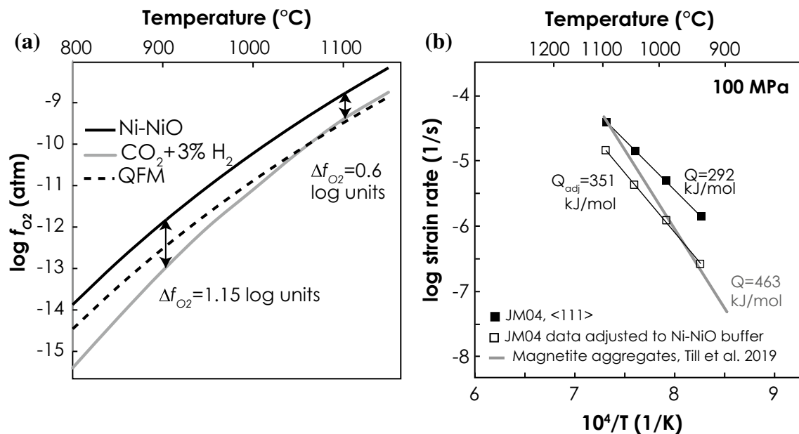
Fig. 9 a Oxygen fugacity curves vs. temperature for different buffers used in magnetite deformation experiments. Values for quartz–fayalite–magnetite (QFM) and Ni–NiO are from Myers and Eugster (1983) and Huebner and Sato (1970), respectively, and oxygen fugacity values for the \text{CO}_2 - \text{H}_2 gas mixture are from Prunier and Hewitt
