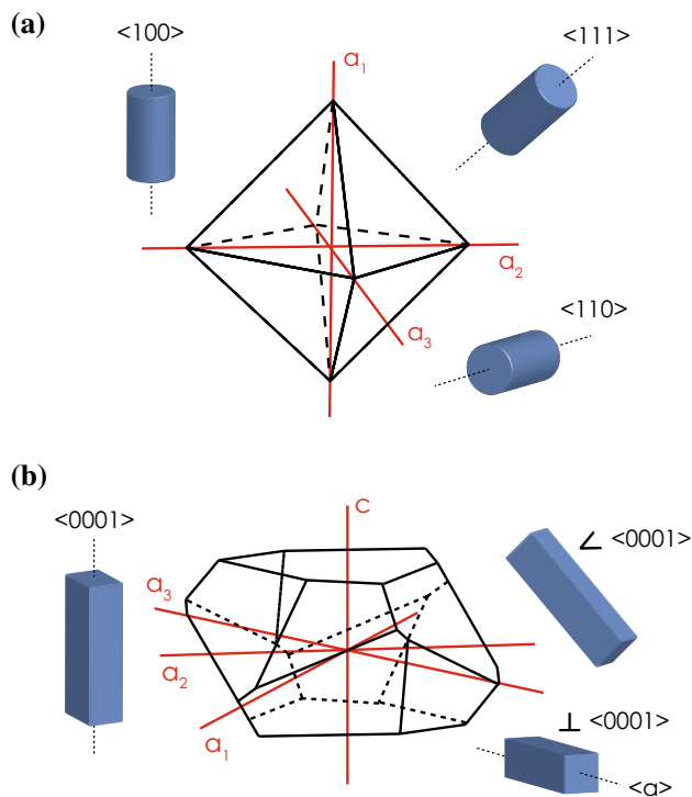
Fig. 1 Diagrams illustrating sample orientations used for creep experiments from a magnetite and b ilmenite single crystals
