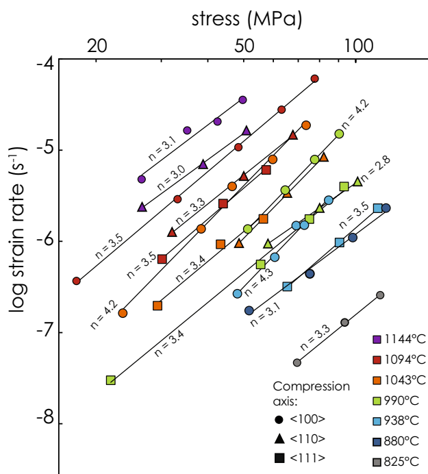
Fig. 4 Log–log plot of strain rate vs. differential stress results for magnetite single-crystal creep experiments at various temperatures. Stress exponents are indicated for each temperature step
