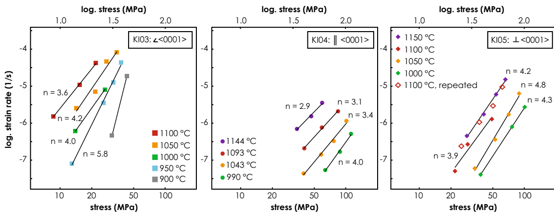
Fig. 6 Log–log plot of strain rate vs. differential stress for ilmenite single-crystal creep experiment results at various temperatures. Stress exponents are indicated for each temperature step.
