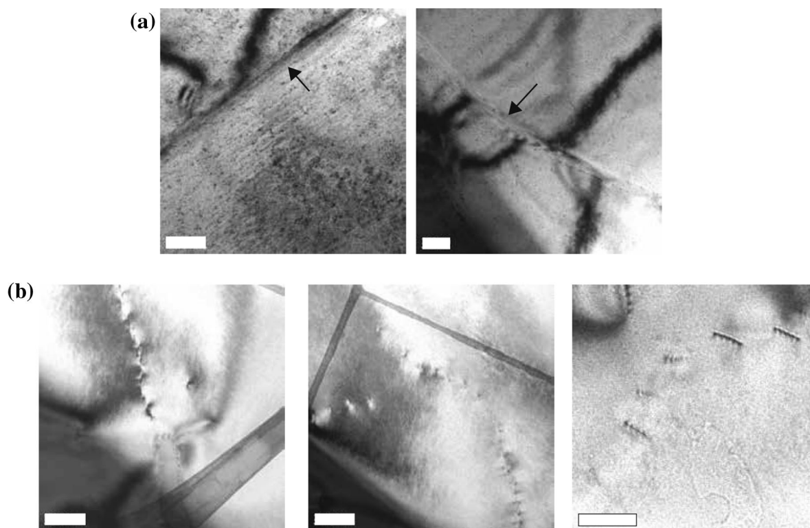
Fig. 3 Transmission electron microscope images of crystalline defects in magnetite and ilmenite. a Slip bands (arrows) in magnetite single-crystal sample JM06 compressed parallel to \langle 100 \rangle ; b dislocations
