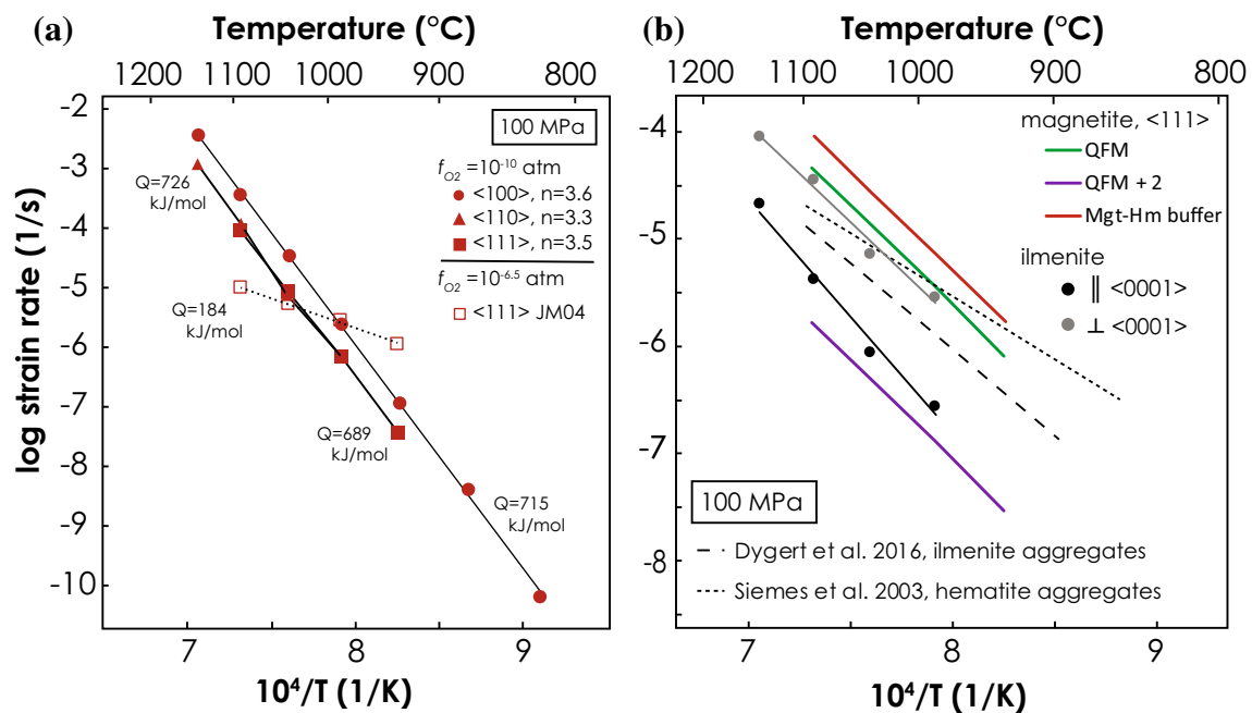
Fig. 11 a Arrhenius plot of magnetite single-crystal creep rates at constant oxygen fugacities. b Plot comparing creep rates for ilmenite compressed along hard orientations with predicted creep rates for magnetite at the quartz–fayalite–magnetite (QFM) buffer, 2 log units
