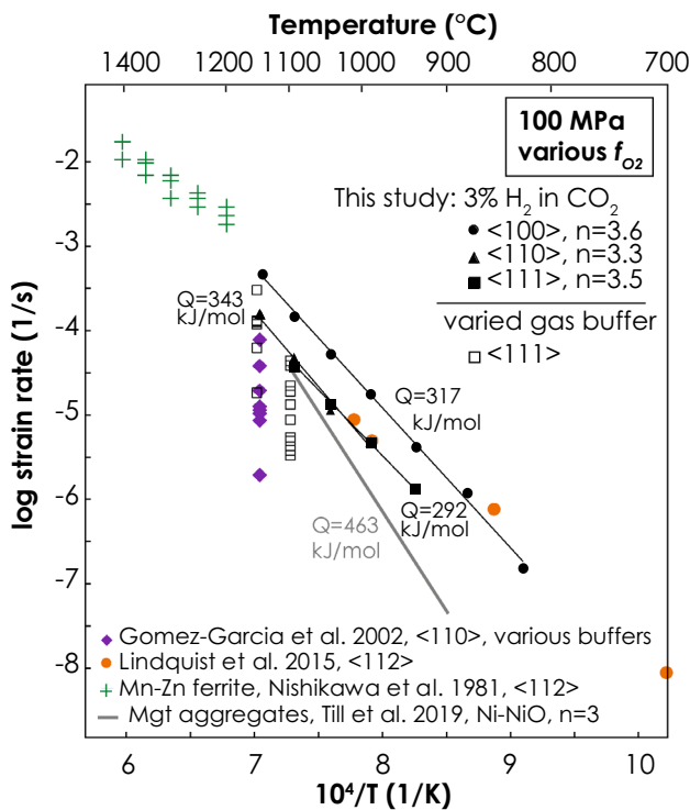
Fig. 5 Arrhenius plot of magnetite single-crystal creep data from this study normalized to a stress of 100 MPa compared with polycrystalline magnetite dislocation creep flow laws from Till et al. (2019). These data sets are labeled with apparent activation energies without accounting for the oxygen fugacity dependence. Previous experimental creep data for single crystals of magnetite and other spinel oxides are also included. Data from experiment JM07 and from Gómez-García et al. (2002) were obtained at various oxygen fugacity buffers, while the other data represent constant f_{O_2} buffers but various absolute f_{O_2} values
