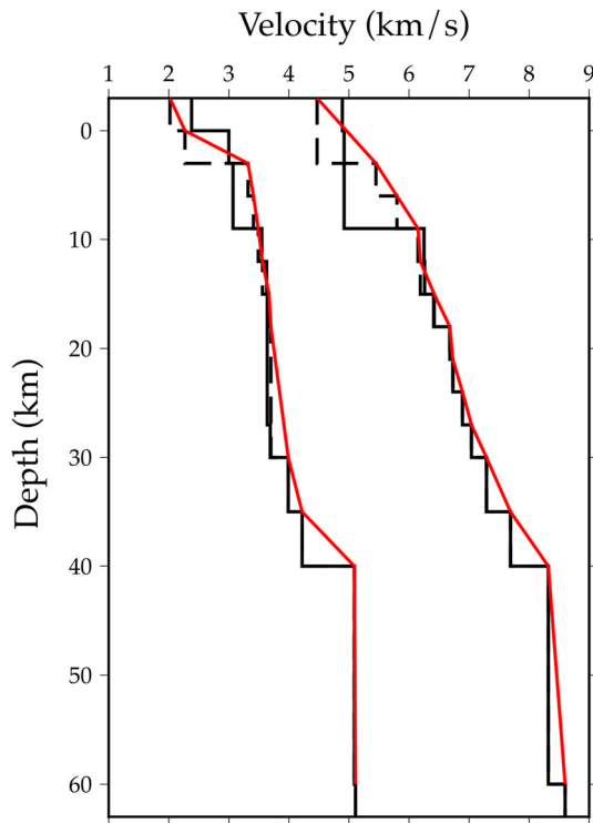
Figure 5. P and Swaves velocity models. The black solid lines represent the model of Sielfeld et al. (2019), the black dashed lines show the velocity model updated for this study, and the red solid lines represent the gradient velocity layers that reduce the sharp discontinuity that occurs at 10 km depth.
