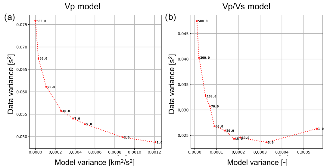
Figure B1. Trade-off curves for (a) V p and (b) V p /V s to select the optimal damping values. The parameters selected were 7 and 10 for V p and V p /V s models, respectively.
