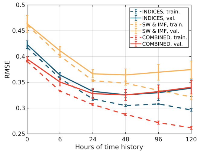
Figure 9. Root-mean-square error (RMSE) on the y-axis versus the hours of time history included in the models. The yellow color shows the errors of models based on solar wind, the blue color is for the models based on geomagnetic indices, and red is for the models based on both of them combined. Solid lines show validation errors and dashed lines show training errors. The error bars show the standard deviation of error on the validation set obtained during the cross validation procedure. RMSE, root-mean-square error.
