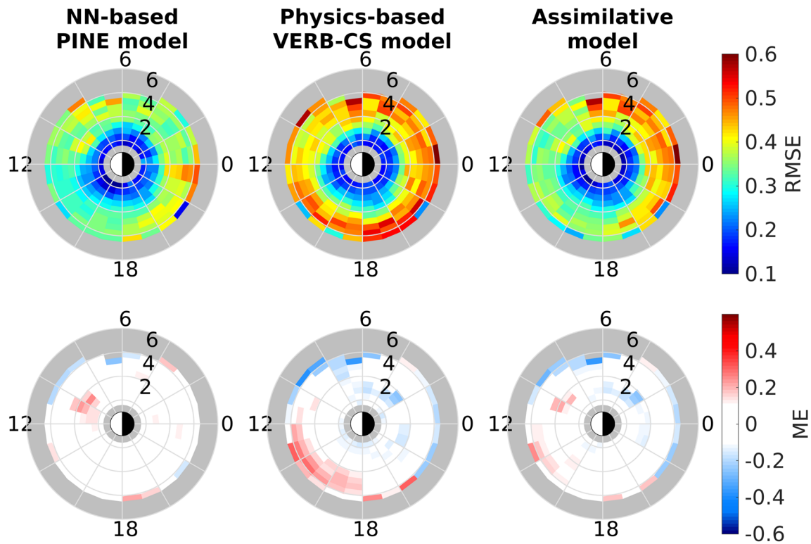
Figure 8. The root-mean-square error (top row) and the bias or mean error (bottom row) of the PINE, physics-based, and assimilative models for the July 02, 2016–January 01, 2018 period. The Sun is to the left. The colorbar of each row shows the value of the corresponding metric (RMSE or ME). The colorbar limits are the same for all models in each row. ME, mean error; RMSE, root-mean-square error.
