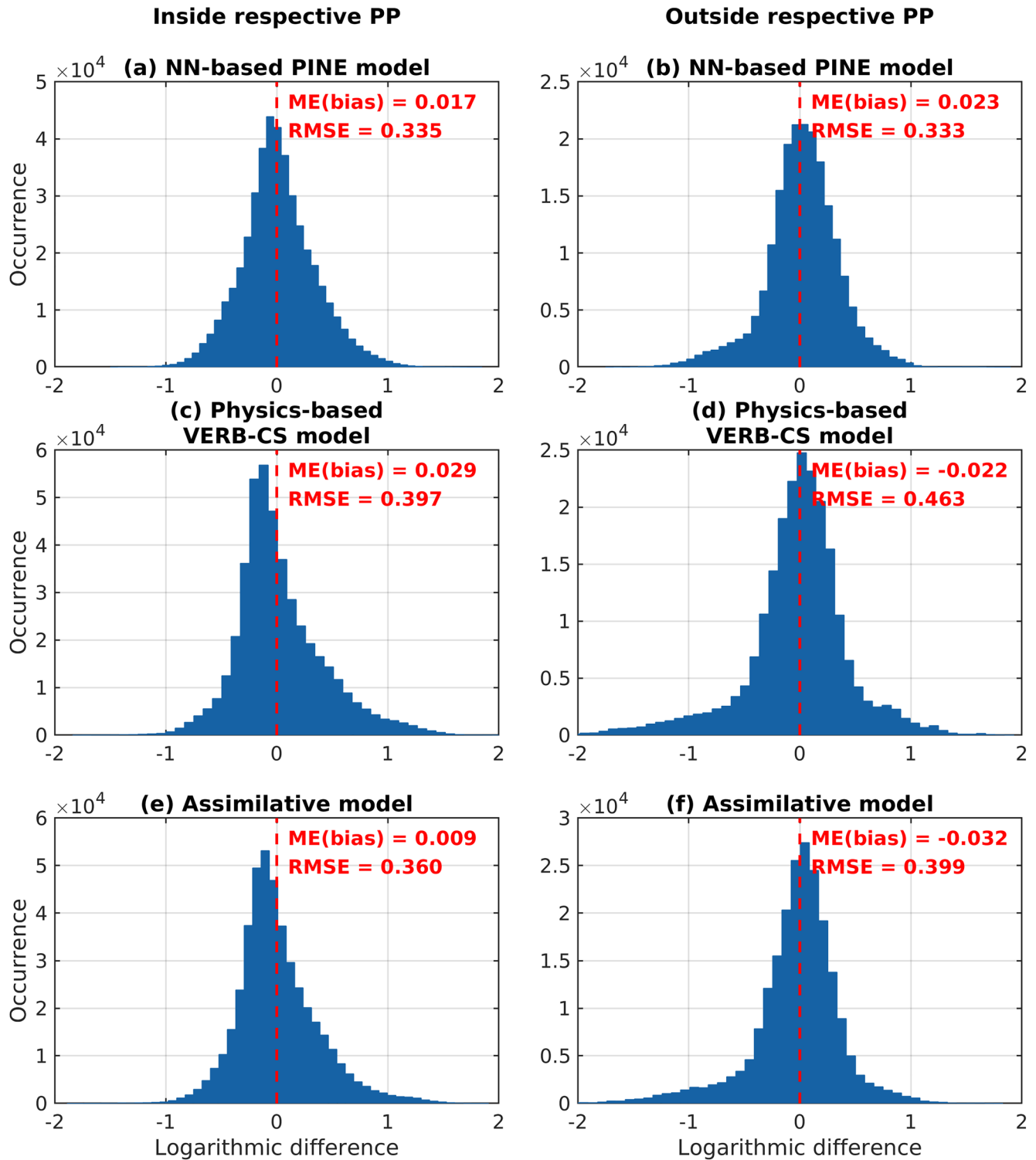
Figure B1. Distribution of errors of PINE, VERB-CS, and the assimilative model inside and outside the plasmopause during the out-of-sample period of July 02, 2016–January 01, 2018 (compared to density measurements from RBSP-A). The respective RMSE and ME are given inside each panel. CS, Convection Simplified; ME, mean error; PINE, Plasma density in the Inner magnetosphere Neural network-based Empirical; RMSE, root-mean-square error.
