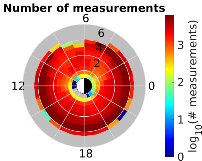
Figure 4. Coverage of RBSP-A during June 30, 2016–January 01, 2018.
