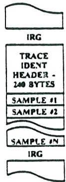
DATA TRACE BLOCK FORMAT 32-BIT IBM FLOATING POINT DATA
