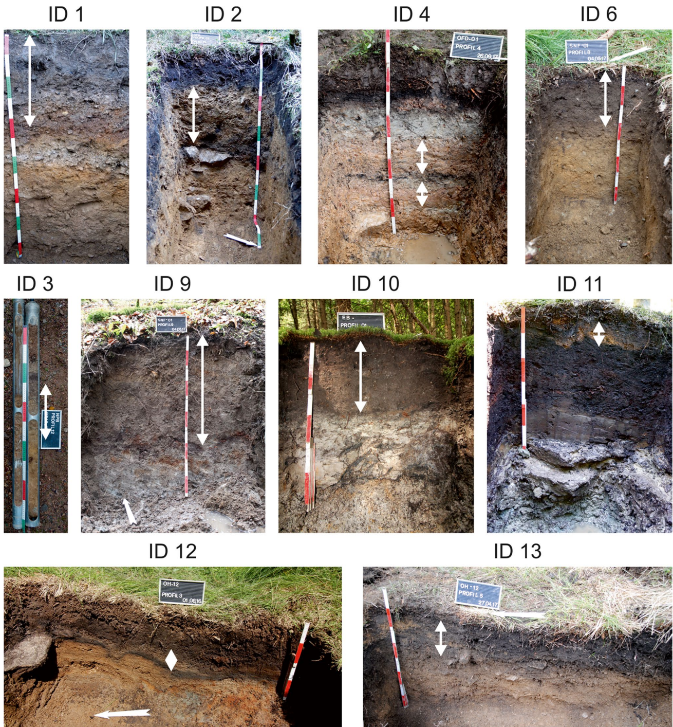
Fig. 4 Photographs of selected sections with colluvial layers in the Erzgebirge Mountains. Colluvial layers are indicated with white arrows. The total length of the ruler varies between 40 and 130 cm. One coloured section is equivalent to 10 cm
