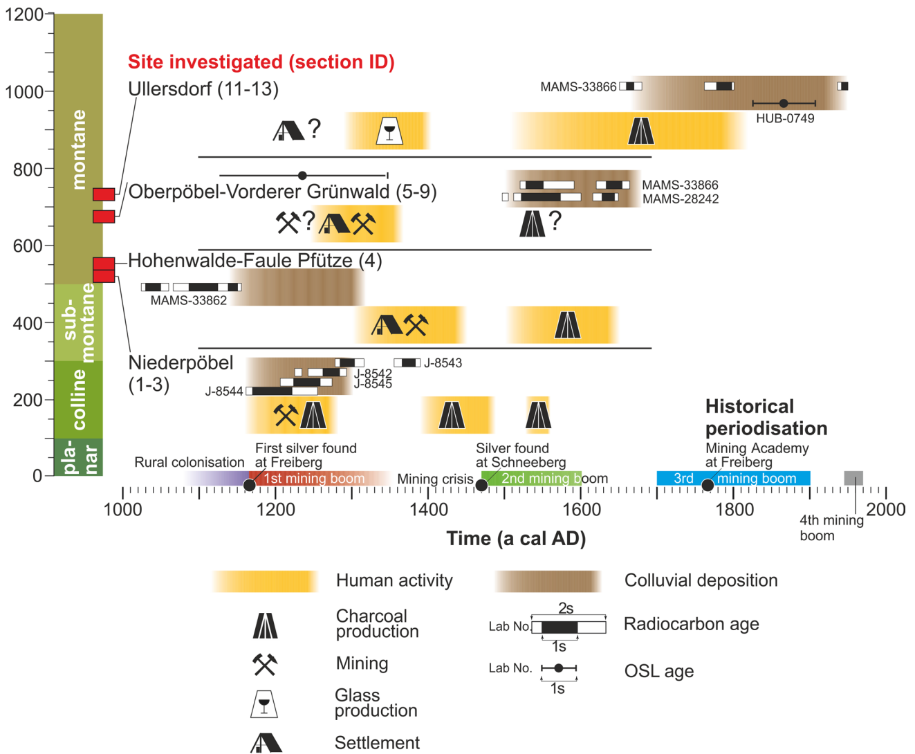
Fig. 7 Synthesis of colluvial dynamics and human activity for the sites investigated at Erzgebirge Mountains. Ecological zonation follows Leuschner and Ellenberg (2017); historical periodisation follows Wagenbreth and Wächtler (1990)
