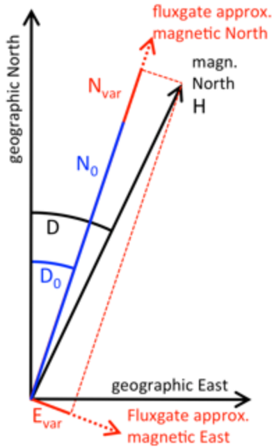
Figure 4 - Horizontal field component H and horizontal sensors of the variometer for the HDZ orientation. See text.
