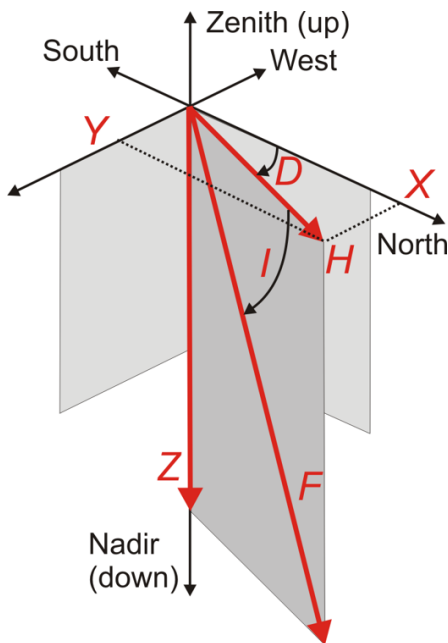
Figure 3 - Geomagnetic components.
