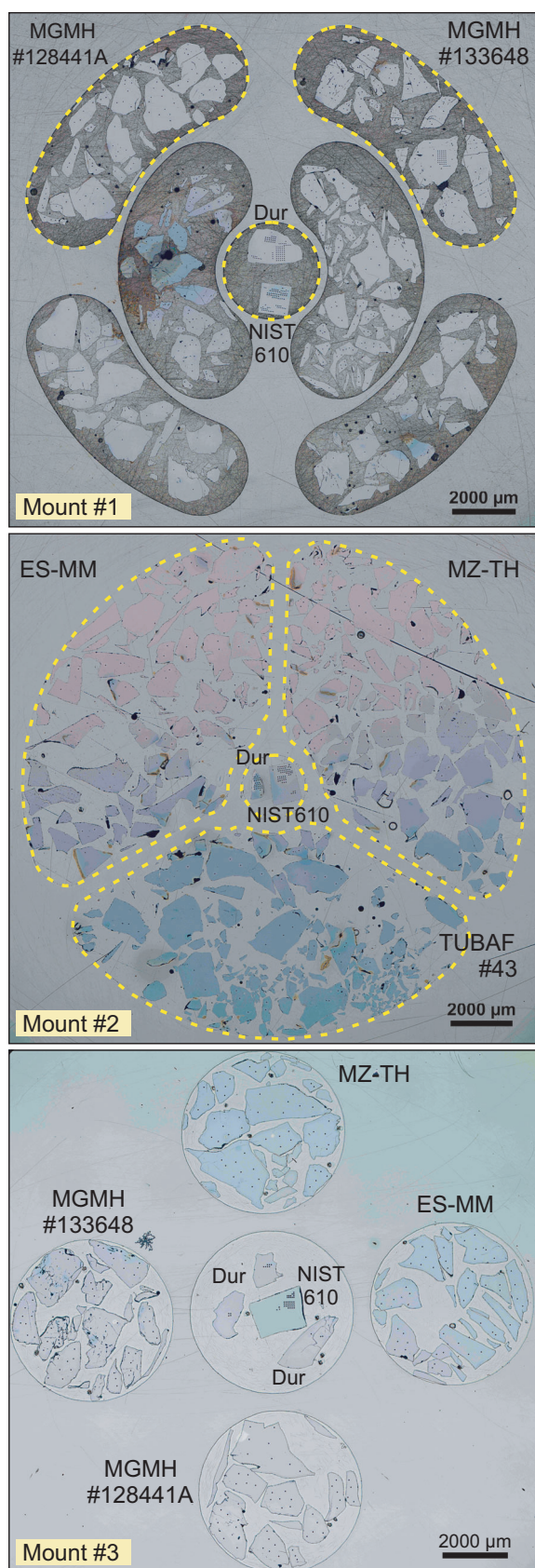
Figure 2. Reflected-light optical images of three gold-coated SIMS mounts. The photographs were taken after SIMS \delta^{18}\text{O} measurements, such that they show the distribution of the analytical spots (black). Mount #1 has previously been used for a chlorine isotope study (Wudarska et al. 2021), and therefore, the analytical spots from \delta^{37}\text{Cl} measurements are also visible in the upper part of the figure. NIST SRM 610 silicate glass and Durango apatite (Dur) were used for tuning purposes and instrumental drift assessment.
