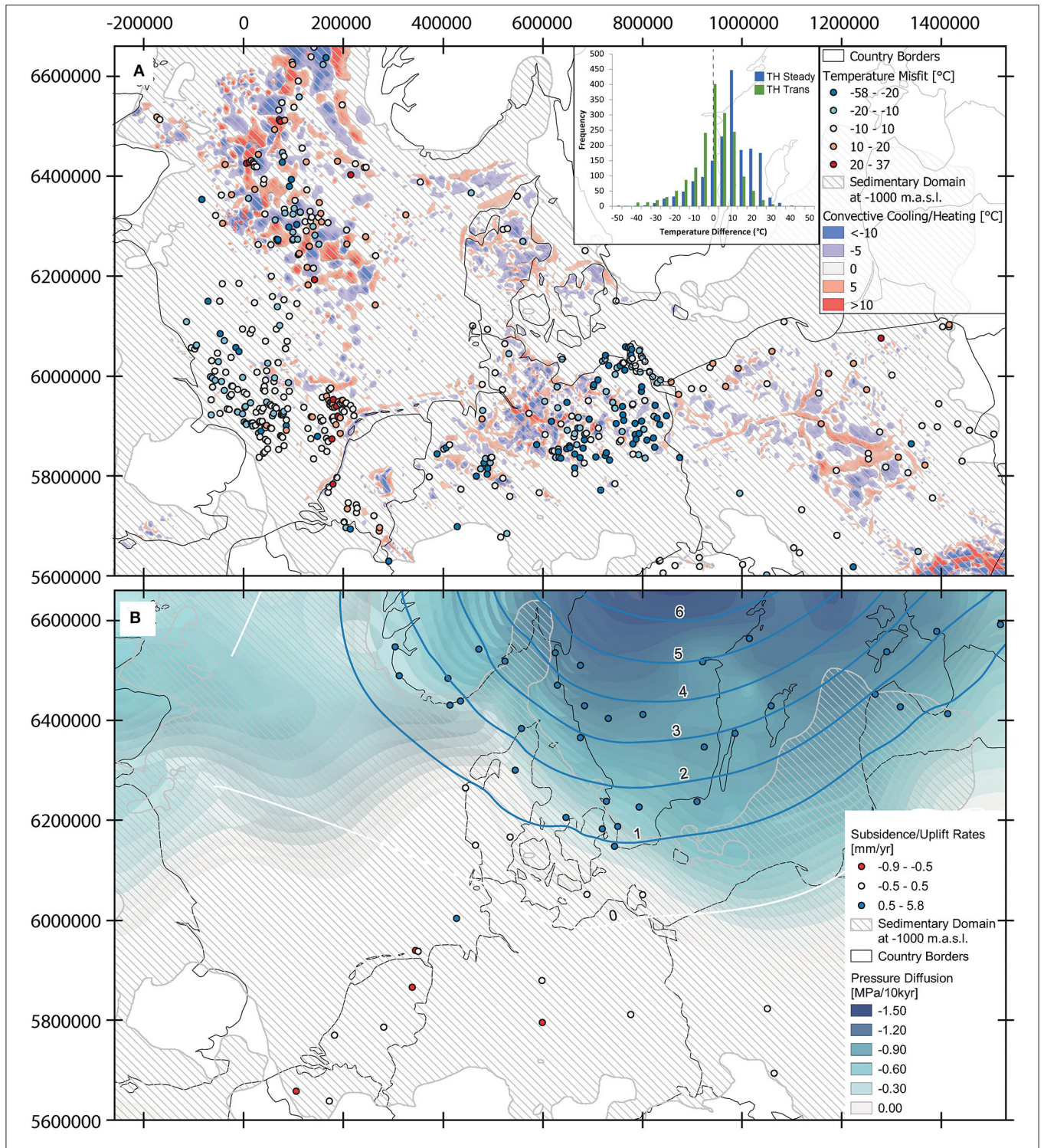
FIGURE 8 | Comparison of modeled data to measured data. (A) Temperature misfit (modeled - measured) between the transient model at present day and available measurements ( Supplementary Material ), blue spheres: model colder than measurements, red spheres: model warmer than measurements. Not all temperature misfits are shown as some localities have more than one measurement vertically. All misfits have been included in the histograms. Backdrop represents influence of convection at -26 kyrs (TH model - T model), inlay: histogram of temperature misfits for the transient model and the steady state model for 0 kyrs (modeled - measured). (B) Circles represent uplift rates at present day after (Vestøl et al., 2019), contour lines represent the empirical model of uplift rates at present day after (Vestøl et al., 2019), backdrop represents the pore pressure dissipation (depth integrated along the model) at present day plotted along in map view to, illustrate its variations in space (A,B) black lines represent the coastline as derived from the 0m contour of the topography distribution of the top slice of the model. Coordinates are in UTM Zone 32N.
