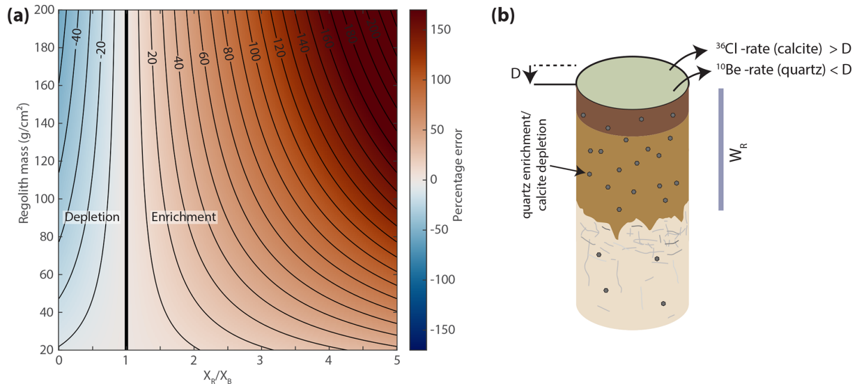
Figure 5. (a) The percentage change in ^{10}\text{Be} concentration compared to a no-weathering case for different regolith masses and ratios of regolith and bedrock mineral fractions ( X_R/X_B ) at sea level high latitude (SLHL). (b) Conceptual representation of a rock with carbonate and quartz minerals experiencing regolith weathering. The quartz grains would be enriched in the regolith compared to the calcite. Therefore, a ^{10}\text{Be} denudation rate computed from quartz without correction would be lower than the average denudation rate, whereas a ^{36}\text{Cl} denudation rate measured from calcite would be higher.
