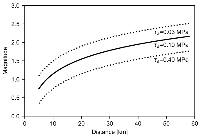
Figure 10. Magnitude detection threshold (with probability 90% at SNR = 2 ) as a function of the distance, for three values of the apparent stress. These values represent the median and 68.8% confidence limits of the apparent stress values for the Irpinia region (Zollo et al., 2014).
