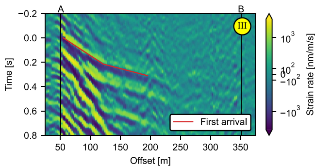
Figure 6. Picking of the first arrival (red line) on the first half of the AB section for the S onset of event III. In first approximation, this gives the difference of travel time to cross all the sedimentary layers at each offset. P onset of events I and II can be seen online (Figure S4 in Supporting Information S1).
