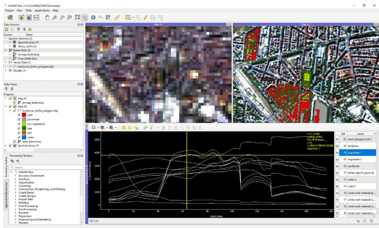
Fig. 7: Graphical user interface of the EnMAP-Box 3, showing simulated EnMAP data linked to map view with very high-resolution data and a vector layer, as well as the associated spectral library viewer.
