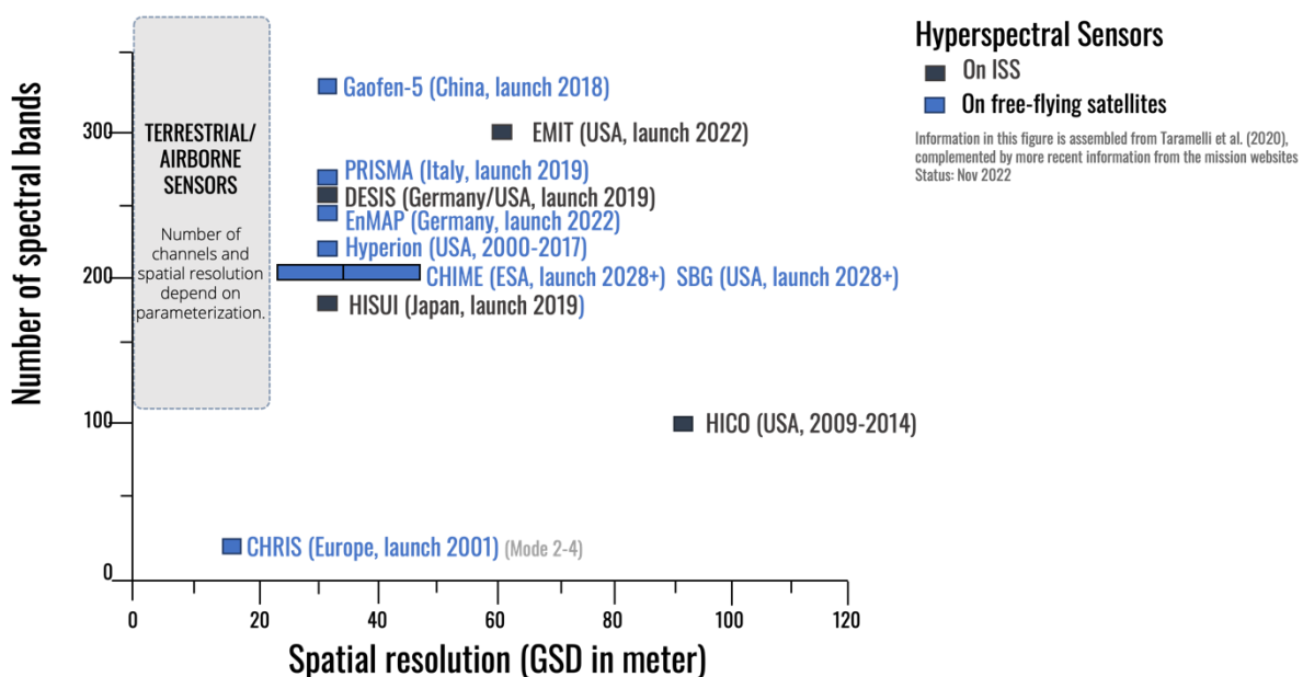
Fig. 3: Overview of the spectral and spatial resolution of airborne sensors and spaceborne hyperspectral missions.
