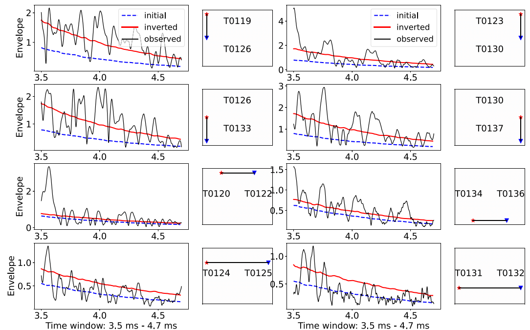
Figure 8. The data fitting of different combinations (illustrated on the right side, red star and blue inverted triangle are source and receiver, respectively) in the later coda wave (3.5–4.7 ms). The blue dashed and red solid curves indicate the envelopes simulated in the initial model and the inverted model shown in Figure 7b, respectively. The black curve is the real data from the concrete experiment.
