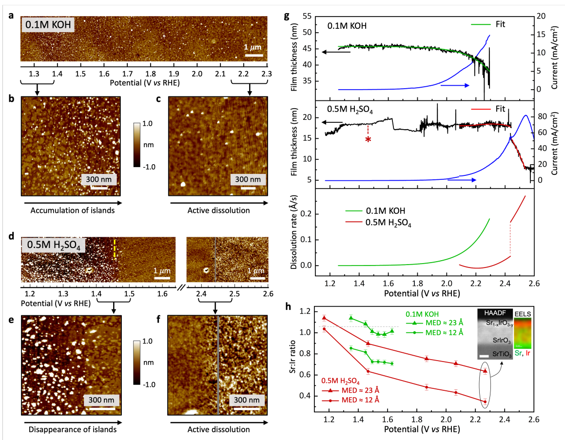
Figure 2. (a) Operando EC-AFM measurements of the \text{SrIrO}_3 film in 0.1M KOH (see also Figure S9). (b, c) An enlarged region of the AFM image showing (b) the initiation of the potential-dependent surface evolution that generates particulates on the surface without the loss of the step-terraced surface morphology, and (c) the dissolution regime (the image is flattened for clarity). (d) The evolution of the \text{SrIrO}_3 film in 0.5M \text{H}_2\text{SO}_4 (see also Figure S10). (e,f) Disappearance of particulates from the surface and the beginning of active dissolution of \text{Sr}_{1-x}\text{IrO}_3 . (g) Evolution of the film thickness in 0.1M KOH and 0.5M \text{H}_2\text{SO}_4 with potential obtained in the operando EC-AFM experiment. The dissolution rate is evaluated by fitting the thickness as a function of time (green curve – exponential fit, red curve – 3 rd degree polynomial fit). The red asterisk marks the potential at which the particulates on the surface in (d) disappear (yellow dashed line). (h) X-ray photoelectron spectroscopy showing Sr depletion at the surface near the OER onset potential for the two electrolytes. MED – mean escape depth. The error bars represent standard deviation in
