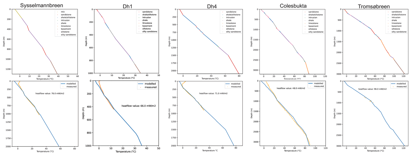
Fig. 15. 1D heatflow models of selected wells, including modelled (blue) and observed (orange) data from Sysselmannbreen, DH4, Colesbukta and Tromsøbreen. The lithologies used in the modelling are highlighted in the upper images.
