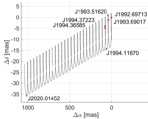
Figure 5.17 Observed positions, selected model in Table 5.12, and adjusted positions for HD 199178. For a description of the plot, see Fig. 5.9.
