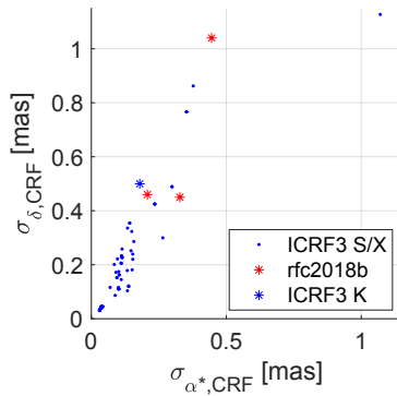
Figure 5.49 Uncertainties of the primary calibrator catalog positions \sigma_{\text{CRF}} = \sqrt{\sigma_{\alpha^*,\text{CRF}}^2 + \sigma_{\delta,\text{CRF}}^2} in directions of \alpha^* and \delta for all observations in “60,EDR3,GA,NM”. The uncertainty of one primary calibrator (J1832-1035, one position for star HD 167971) with (\sigma_{\alpha^*}, \sigma_{\delta}) of (4.9,5.1) mas from ICRF3 S/X is outside the plot range.
