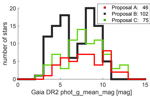
Figure 5.2 Histogram of G-magnitude of the stars selected for the observations.
