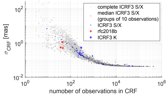
Figure 5.50 Uncertainties of the primary calibrator catalog positions \sigma_{\text{CRF}} = \sqrt{\sigma_{\alpha^*,\text{CRF}}^2 + \sigma_{\delta,\text{CRF}}^2} for all observations of the object in the respective CRF along with the values for all objects in ICRF3 S/X. The dark grey points are the median values of all ICRF3 S/X values per bin of 10 observations. The axes are logarithmic.
