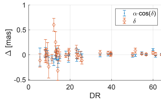
Figure B.4 Differences between the positions from the AIPS task JMFIT and the modelfit functionality from Difmap for the detected stars, sorted by the dynamic range DR from AIPS.
