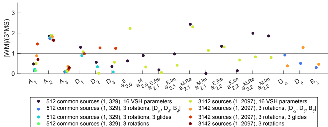
Figure 4.66 Significance of the transformation parameters, (a) between ICRF3 S/X and Gaia DR2, (b) between ICRF3 S/X and Gaia EDR3. If the value of WM/(3MS) is larger unity, the parameters are considered as significantly determined. The results are shown for the various transformation methods as shown in Figs. 4.63 and 4.65.
