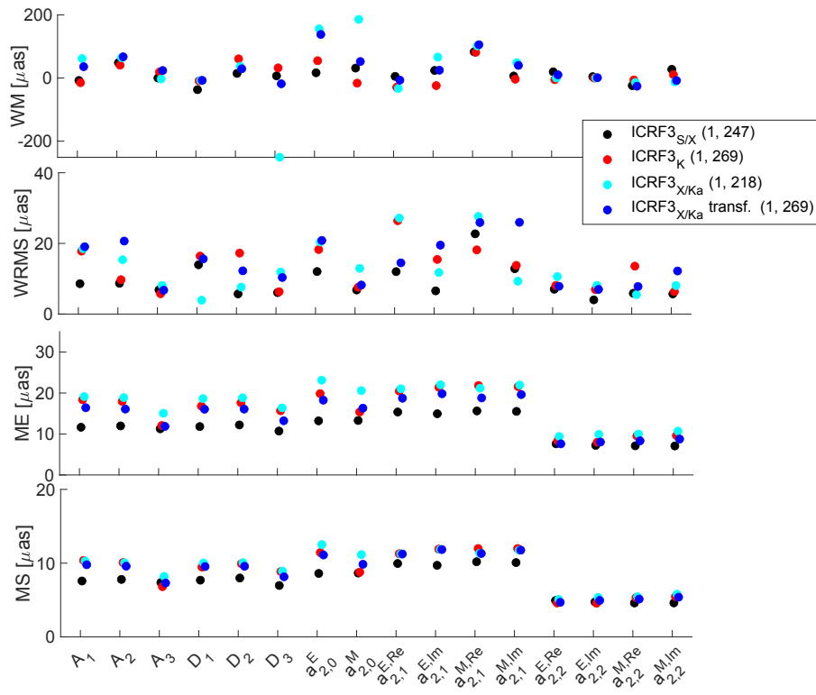
Figure 4.59 WM, WRMS, ME, and MS quantities for the iterative results for the 16 VSH parameters between the various VLBI-based CRFs and (a) Gaia DR2 or (b) Gaia EDR3. Only the 406 counterparts common to all these CRFs were used to have comparable results, and only the counterparts which are not outliers according to their normalized arc lengths were selected. Thus, the number of counterparts differs slightly for Gaia DR2 and Gaia EDR3. In the legend, the numbers in parentheses indicate the start and end of the iterations used to derive the quantities. Typically, this is the first iteration and the number of suitable counterparts minus the last 20% of the iterations (to mitigate any effects due to low number of counterparts in those iterations).
