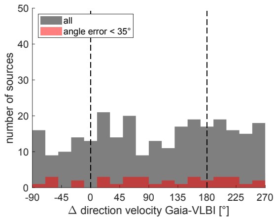
Figure 4.68 Comparison of the selected linear apparent proper motions for 275 AGN from Gaia DR2 and CRFGT based on the weighted RANSAC. For the 625 suitable sources for CRF7918 there is also no clear dependency.
