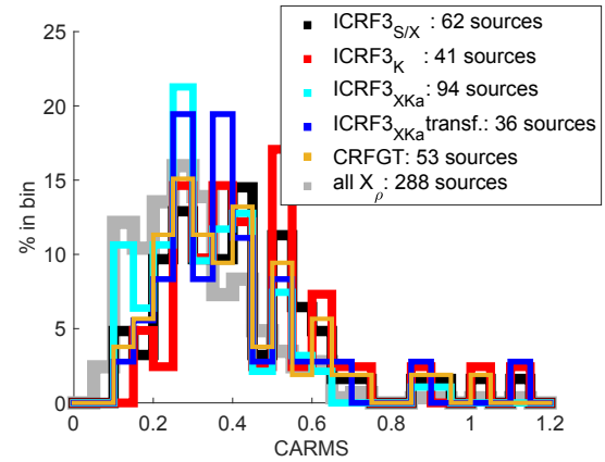
Figure 4.39 Histogram of CARMS values based on basic-noise weighting for radio sources with at least 70 observations in each of the VLBI-based CRFs. The grey line depicts the histogram for all 288 counterparts (288 out of the 289 counterparts have CARMS values), while colored histograms depict the sources of the various CRFs with X_\rho > 3.6 . 22 % of the 288 sources have CARMS > 0.4 , while for sources with X_\rho > 3.6 it is between 27 % and 51 %.
