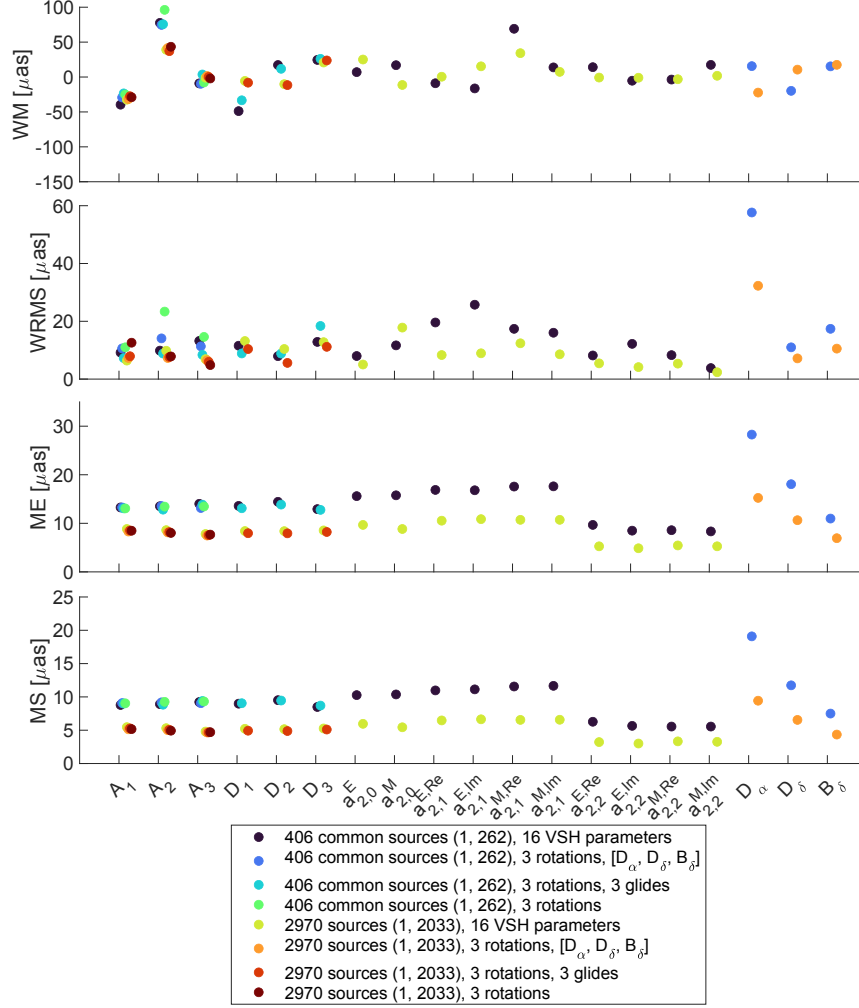
Figure 4.63 WM, WRMS, ME, and MS quantities for the various transformation parameters between ICRF3 S/X and Gaia DR2. Two sets of counterparts were tested: the 406 counterparts common to all VLBI-based CRFs and Gaia DR2 or the 2970 counterparts between ICRF3 S/X and Gaia DR2. Only counterparts for which the normalized arc lengths are not outliers were used. The first iteration and the number of suitable counterparts minus the last 20% of the iterations (until iteration 262 or 2033) was used to mitigate any effects due to low number of counterparts in those iterations.
