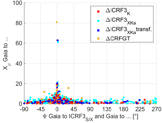
Figure 4.46 Angle differences \Psi as in Fig 4.41a versus the normalized arc lengths X_\rho between the Gaia DR2 and respective CRF positions for the 289 radio sources with more than 70 observations in each of the VLBI-based CRFs.
