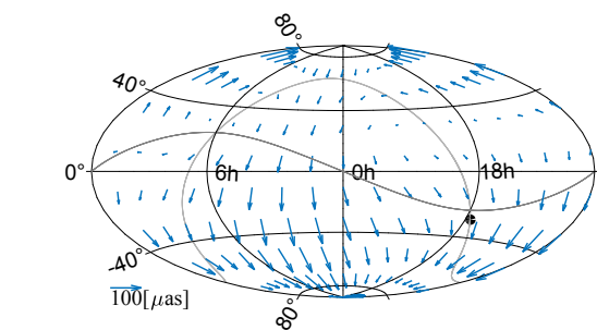
Figure 4.23 Sky plot of the combined global systematic differences in terms of VSH for a set of evenly distributed source positions (to better visualize the pattern) between (a) ICRF3 K and ICRF3 S/X, (b) CRF7918 and ICRF3 S/X, and (c) CRFGT and ICRF3 S/X.
