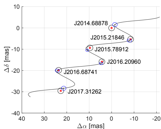
Figure 5.21 Observed positions, selected model in Table 5.12, and adjusted positions for CoKu HP Tau G2. For a description of the plot, see Fig. 5.9.
