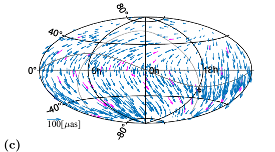
Figure 4.22 Sky plot of the combined global systematic differences in terms of VSH between ICRF3 X/Ka and ICRF3 S/X for (a) a set of evenly distributed source positions (to better visualize the pattern) and (b) the actual sources used to determine the VSH terms (blue) and the initially removed outliers with respect to their normalized arc length X_\rho (magenta). (c) gives a similar plot to (b), except that the differences are shown for ICRF3 X/Ka already transformed to ICRF3 S/X (labelled “ICRF3 X/Ka transf.” in this work). Thus, it is a new iteration of the transformation to ICRF3 S/X with a new set of outlier sources. Note the difference in scale compared to (a) and (b).
