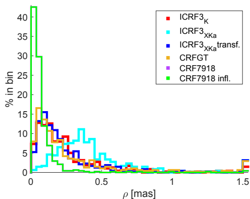
Figure 4.8 Arc lengths \rho for the 477 sources common to the various VLBI-based CRFs versus ICRF3 S/X.
