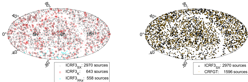
Figure 4.4 Sky distribution of the counterparts between various VLBI-based CRFs and Gaia DR2. Figure 4.5 Sky distribution of the counterparts between ICRF3 S/X or CRFGT and Gaia DR2.
