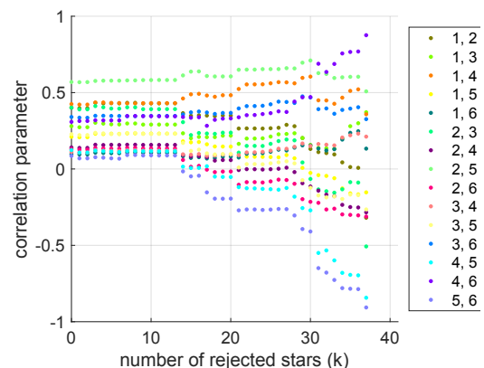
Figure 5.30 Correlation parameters for all iterations of “41,EDR3”. The numbers 1 to 6 represent the rotation parameters in the order [\epsilon_X(T), \epsilon_Y(T), \epsilon_Z(T), \omega_X, \omega_Y, \omega_Z] .
