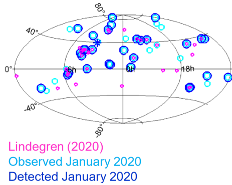
Figure 5.7 Sky plot of the Lindegren (2020a) stars, the observed stars, and the detected stars in January 2020 (this work). Note. According to Lunz et al. (2021a).
