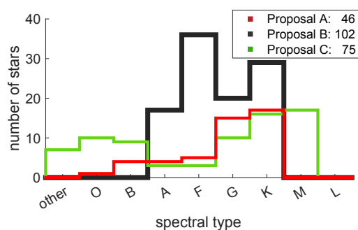
Figure 5.3 Histogram of the spectral types of the stars selected for the observations. For proposal C, a stricter selection for the most suitable spectral types would be possible.
