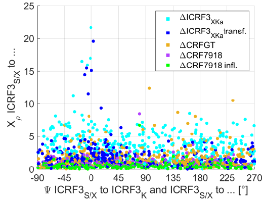
Figure 4.19 Angle differences \Psi as in Fig. 4.18a versus the normalized arc lengths X_\rho between the ICRF3 S/X and respective CRF positions for the 333 radio sources with more than 70 observations in each of the CRFs.
