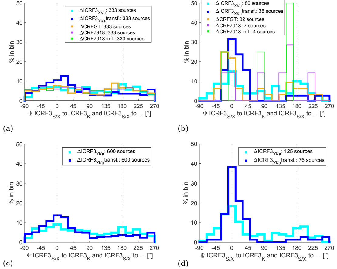
Figure 4.18 Position angle differences \Psi between the arc from the ICRF3 S/X position to the ICRF3 K position versus the other CRFs, as listed in the legend, (a) for radio sources with at least 70 observations in each of the CRFs (333 counterparts), (b) same as (a) but with an uncertainty of \Psi smaller than 30^\circ , (c) for radio sources common to all ICRF3 catalogs (600 counterparts), (d) same as (c) but with an uncertainty of \Psi smaller than 30^\circ .
