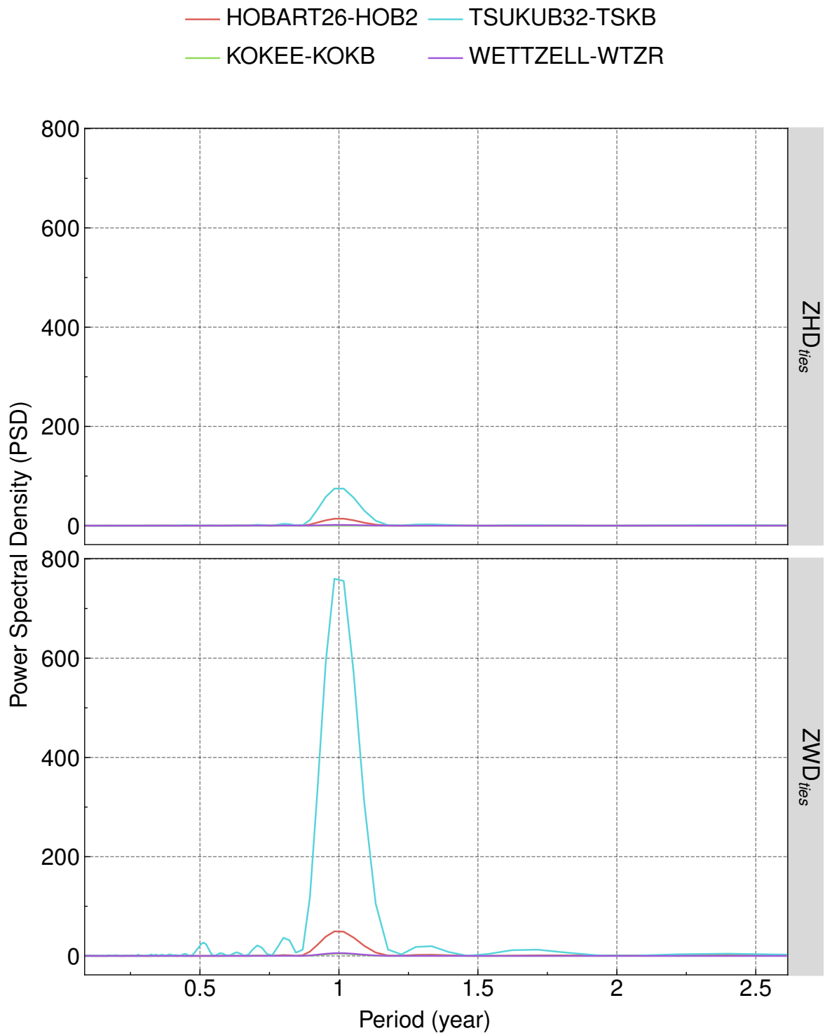
Figure 3.8: The power spectral density (PSD) of the periodic signal in the tropospheric ties was estimated from the Lomb-Scargle periodogram (Lomb, 1976; Scargle, 1982) for both ZHD (top) and ZWD (bottom) between VLBI and GNSS at four co-location sites between 2008 and 2014. These sites include Wettzell (WETTZELL-WTZR), Germany (with a height difference of 3.5 m); Hobart (HOBART26-HOB2), Australia (with a height difference of 24.5 m); Tsukuba (TSUKUB32-TSKB), Japan (with a height difference of 18.6 m); and Kokee Park (KOKEE-KOKB) (with a height difference of 9.5 m), USA. The tropospheric ties were derived from TAVM3.
