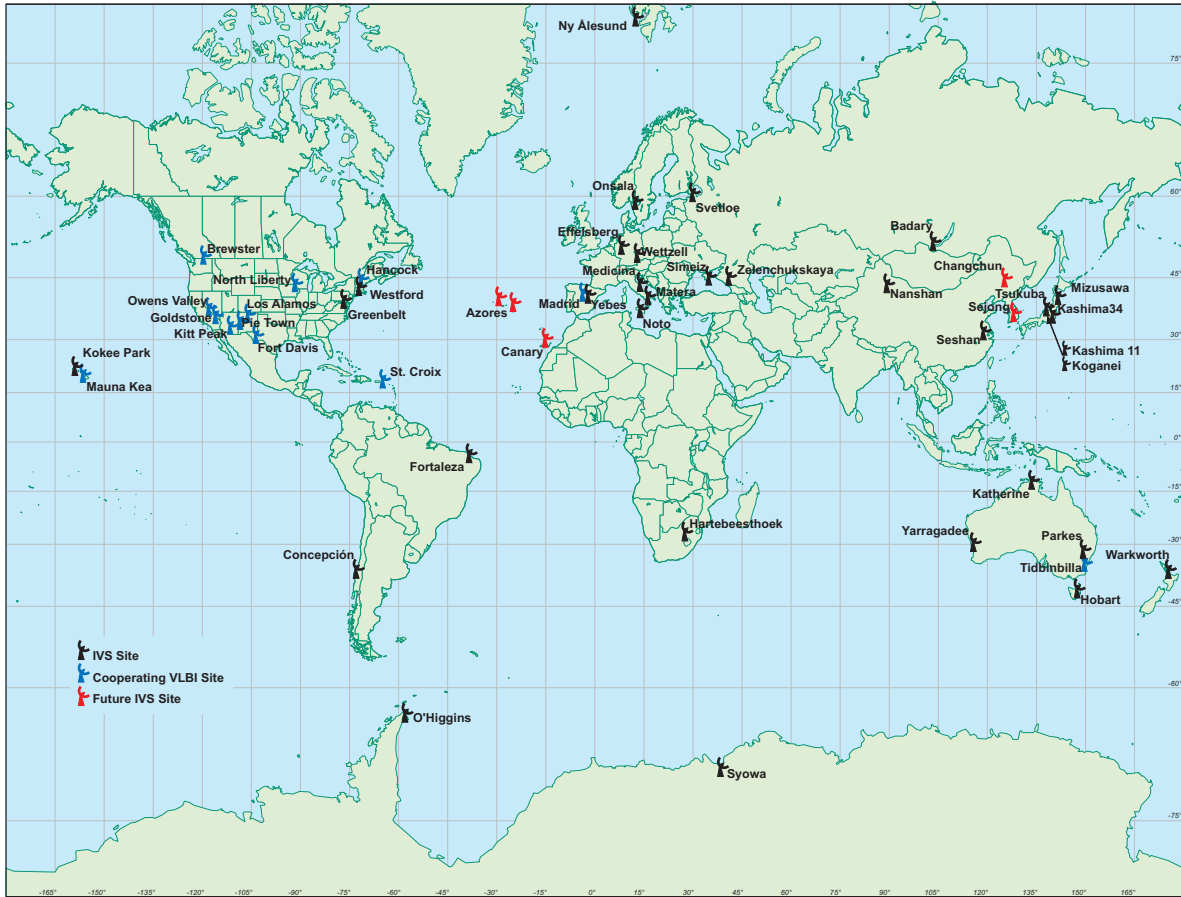
Figure 2.3: Locations of the 40 VLBI radio telescopes in the global network of the IVS (Courtesy from IVS).
