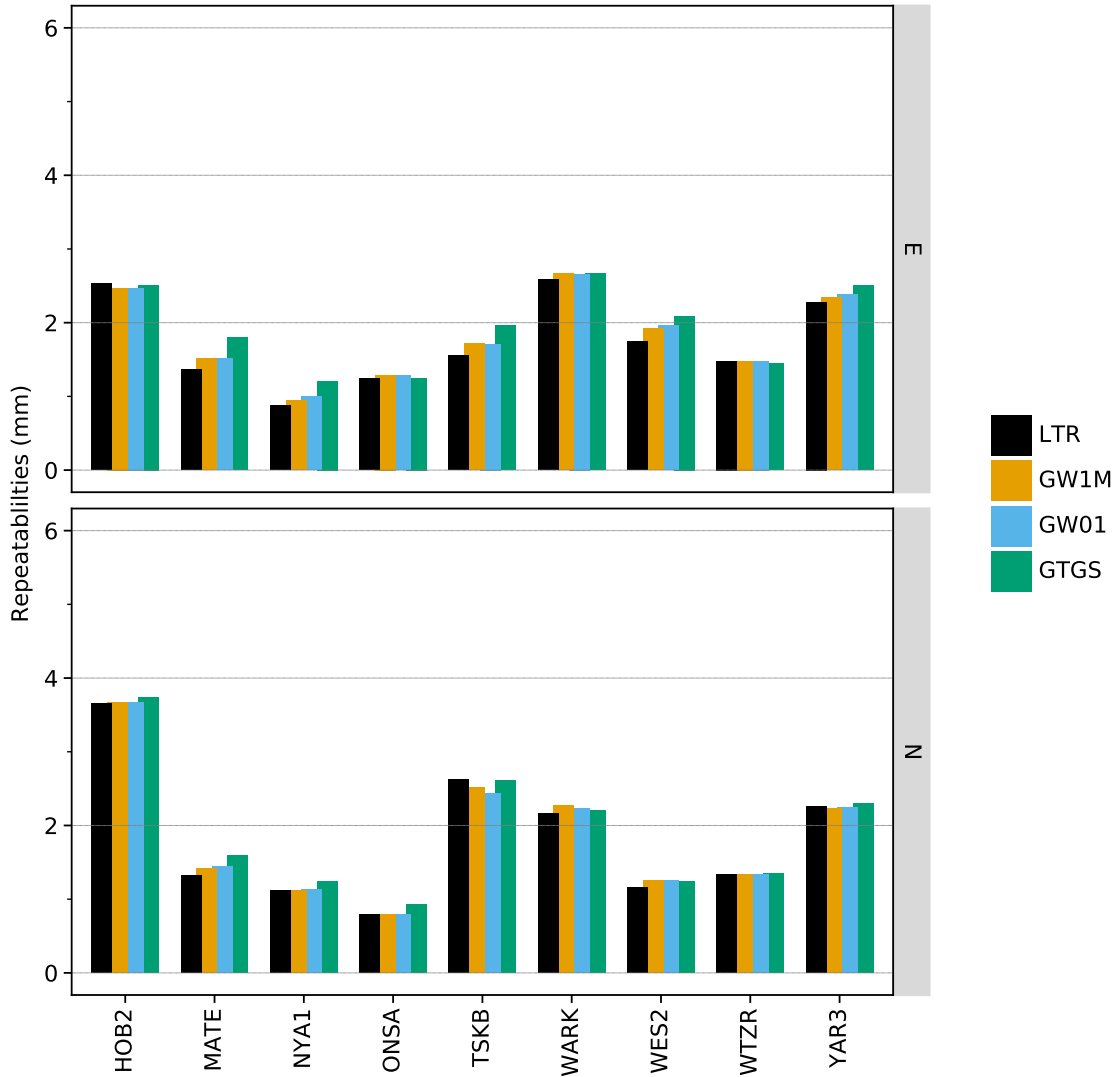
Figure 5.4: GNSS horizontal coordinate repeatabilities of co-location sites where the horizontal component of local ties is questionable, as well as two co-location sites (Wetzell and Yarragade) where the horizontal component of local ties is of good quality, derived from a station-wise combination utilizing gradient ties with three different weightings with respect to the reference solution (LTR).
