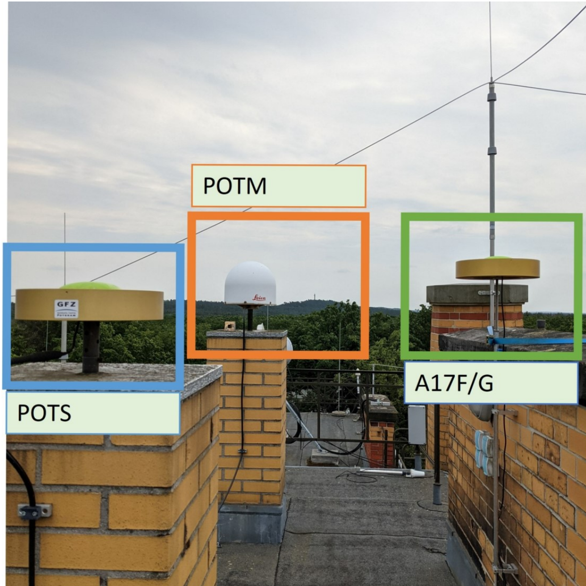
Figure 4.4: The GNSS co-location experiment set-up on the rooftop of A17 building (Telegrafenberg, Potsdam Germany). Two permanent GNSS stations, namely POTS and POTM, were placed on a similar level and continuously operated. The experimental station A17F/G was attached to a vertical steering pole that allows the mitigation of height shift when changing the antenna during the experiment. The picture was taken from Kitpracha et al. (submitted)).
