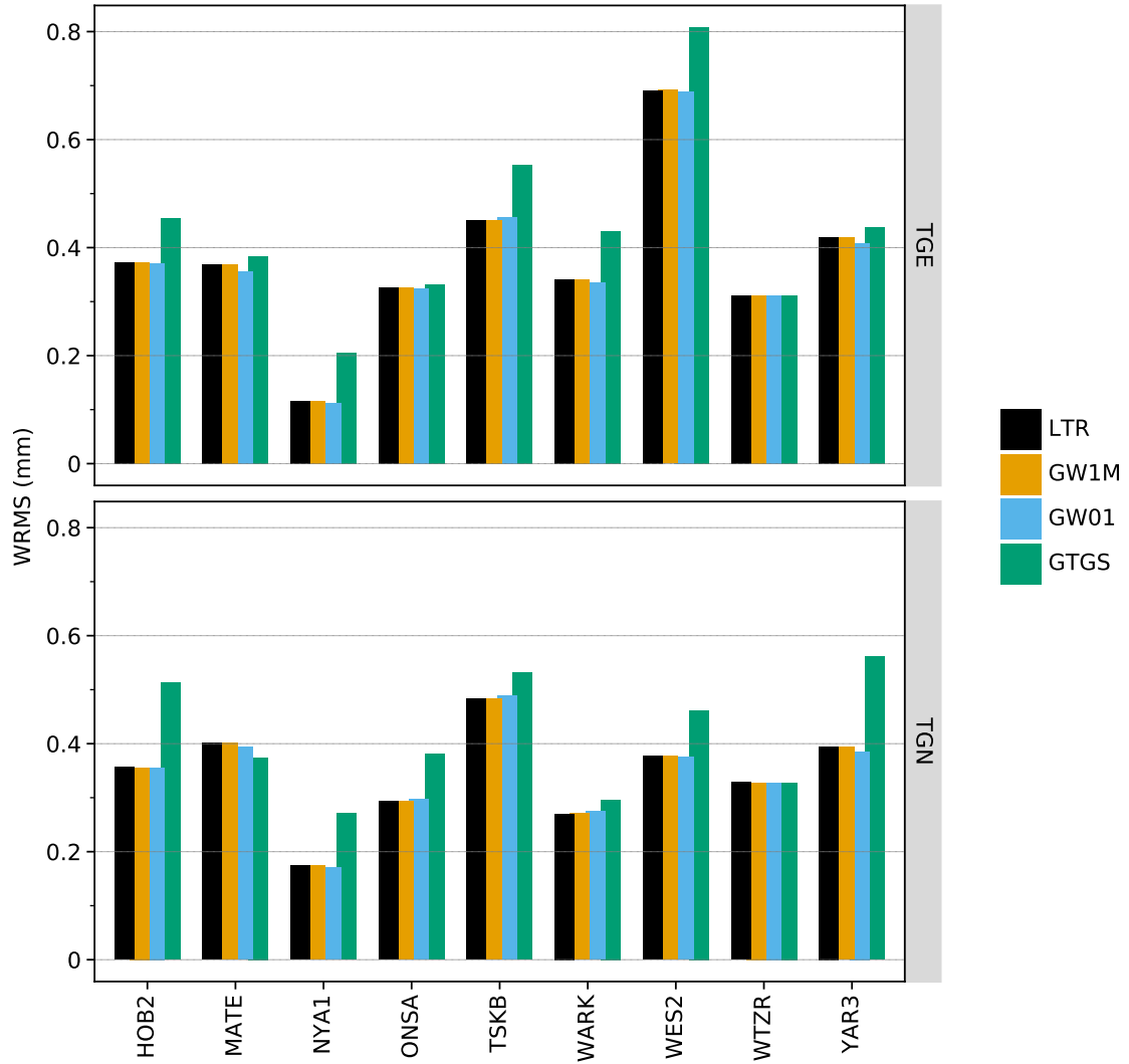
Figure 5.11: WRMS of horizontal gradient parameters w.r.t. ERA5 NWM of GNSS co-location sites where the up component of local ties is questionable, as well as two co-location sites (Wetzell and Yarragade) where the up component of local ties is of good quality, derived from a station-wise combination utilizing gradient ties with four three weightings with respect to the reference solution (LTR).
