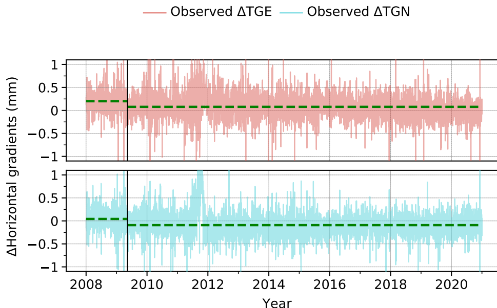
Figure 3.18: The time series depicts observed horizontal gradient differences between two GNSS stations at the Zimmerwald co-location site, namely ZIMM and ZIM2. The horizontal distance between them is approximately 2 meters. The antenna change events (black solid line) are also shown. The green dashed line shows the mean offset for each antenna. The terms \Delta TGE and \Delta TGN refer to the differences in east and north gradients, respectively.
