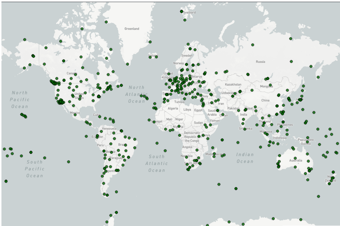
Figure 2.4: Locations of the more than 500 GNSS stations of the global tracking network of the IGS as of September 2023 (Courtesy from IGS).
