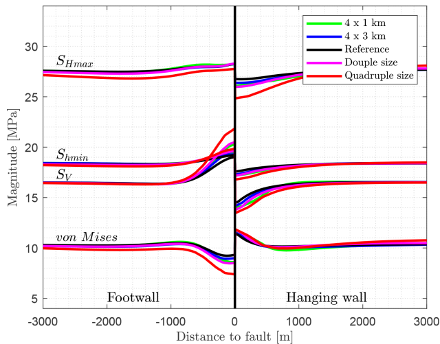
Figure 22. Influence of the fault size on the stress components S_{Hmax} , S_{hmin} , and S_V , as well as the von Mises stress. Models with a reduced fault surface area with a size of 4 \times 3 and 4 \times 1 \text{ km}^2 (Fig. 21), as well as models like the reference model with a total size of 20 \times 20 \times 6 \text{ km}^3 (double size) and 40 \times 40 \times 12 \text{ km}^3 (quadruple size), are shown.
