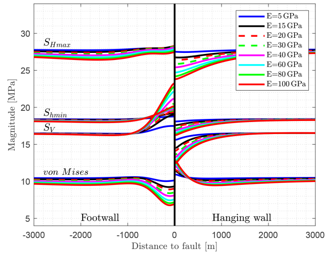
Figure 20. The influence of Young’s modulus on the stress perturbation is investigated. The models have a Young’s modulus of E = 5, 15 (reference model), 20, 30, 40, 60, 80, and 100 GPa.
