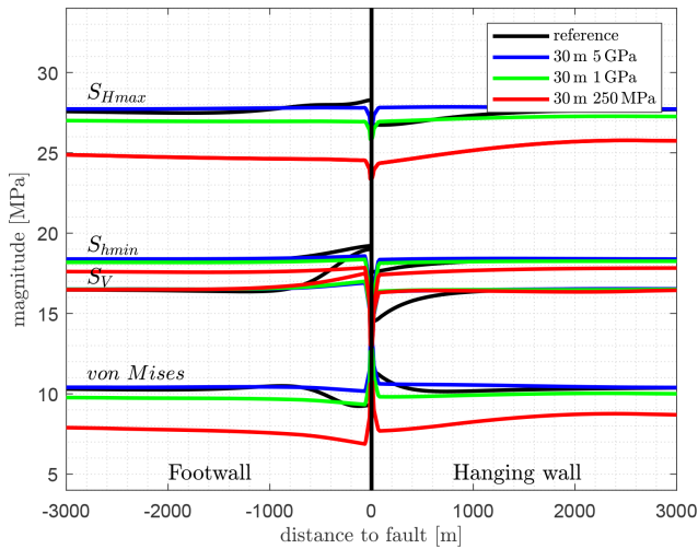
Figure 11. Fault representation by 30 m (nine elements) of elastic weak elements having a lower Young's modulus ( E = 5, 1, and 0.250 GPa) compared to the area outside this region with E = 15 GPa. In colours are the model results with the less stiff 3-D fault representation. Shown in black is the reference model using contact surfaces and vertically the implemented fault zone at 0 m.
