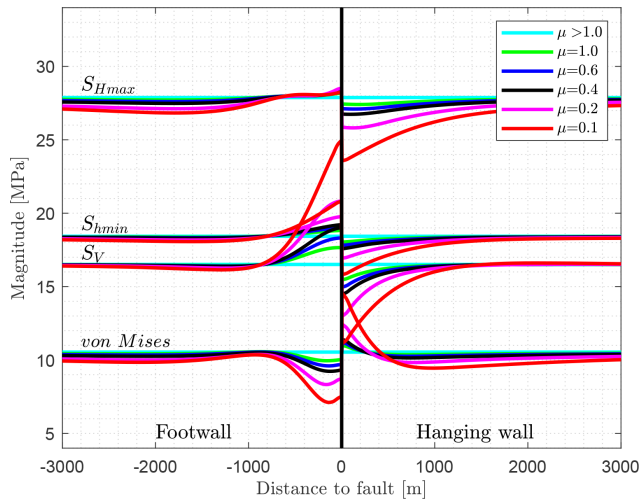
Figure 8. Impact of a variable friction coefficient on the stress state. Plotted are the S_{Hmax} , S_{hmin} , and S_V as well as the von Mises stress. The graph with the friction angle of \mu = 0.4 is the reference model (Fig. 5). Large stress variations near the fault are a result of low friction.
