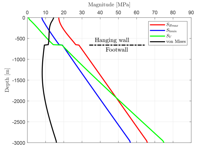
Figure 4. Virtual vertical well path in the centre of the reference model. Shown are the resulting stress components, which are S_{Hmax} , S_{hmin} , S_V , and the von Mises stress. The fault with a friction coefficient of \mu = 0.4 is traversed at a depth of -660 \text{ m} . When crossing the fault from the hanging wall to the footwall block, there is a sudden increase in S_V for S_{Hmax} and for S_{hmin} a little less.
