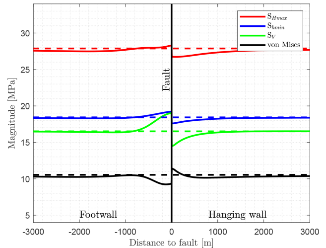
Figure 5. Stress magnitude visualization of the reference model from -3000 m (footwall – left) to +3000 m (hanging wall – right) for a constant depth of -660 m. Linear elastic material properties and a friction coefficient of \mu = 0.4 are used for the fault at 0 m, represented by the vertical black line. The dashed lines in comparison represent results of a similar model without a fault.
