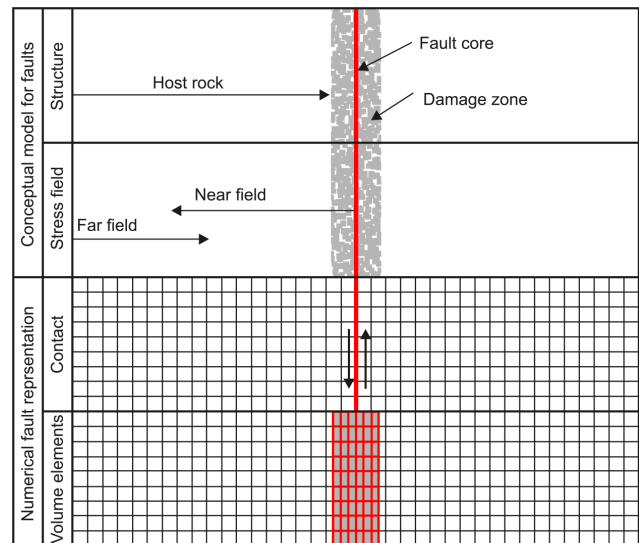
Figure 1. The general structure of a fault is described by the fault core, the damage zone, and the host rock (e.g. Caine et al., 1996; Faulkner et al., 2003). The purpose of this study is not to explore the effect of a fault on the stress state in the near field. This would include the fault core, the damage zone, and the neighbouring host rock. The study is focused on the far-field stress state, which is located several tens or hundreds of metres away from the fault and can extend up to a few kilometres at most. Numerical models typically employ one or a combination of two principle technical fault representations. Contact surfaces are a discontinuity within the mesh, where relative offset of the mesh is allowed, mainly depending on the friction. The second method uses a continuous mesh with elements having a lower stiffness or a failure criterion which results in a distributed deformation within the defined fault representation elements.
