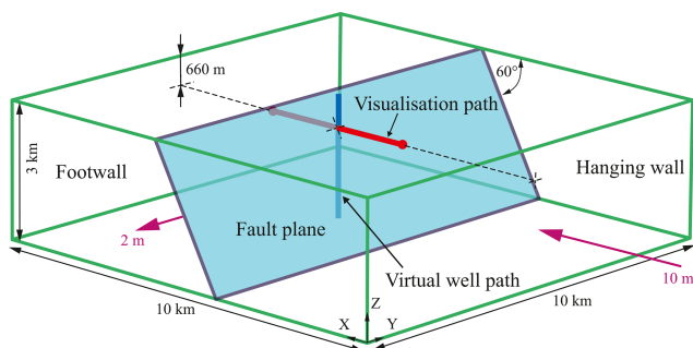
Figure 3. The model extent ( 10 \times 10 \times 3 \text{ km}^3 , in green) with the fault (blue plane) inclined by 60^\circ (dip angle); in red is the visualization path at a depth of 660 m along which the stress magnitudes are presented for the majority of the figures. The vertical blue line indicates the location of a virtual vertical borehole (Fig. 4). The displacement boundary conditions in purple represent 10 m shortening ( \epsilon = -1 \times 10^{-3} ) in the X direction (perpendicular to the strike direction of the fault), which governs the S_{Hmax} magnitude, and 2 m of dilation ( \epsilon = 2 \times 10^{-4} ) in the Y direction (parallel to the strike direction of the fault), which drives the S_{hmin} magnitude.
