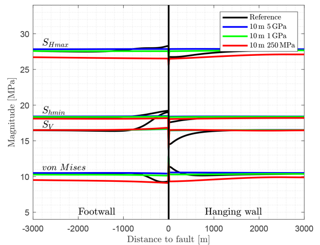
Figure 10. Fault representation by a 10 m thin layer of three weak elements. The fault elements have a lower Young’s modulus ( E = 5, 1, and 0.25 GPa) in contrast to the area outside this region ( E = 15 GPa). Shown in black is the reference model and vertically the implemented fault zone. Stress changes are narrowly limited to the area of the fault so that they are hidden by the visualization of the fault zone.
