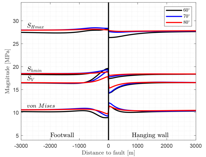
Figure 15. Influence of the dip angle of the fault on the stress components S_V , S_{Hmax} , and S_{hmin} , as well as the von Mises stress. Shown are the models with a fault dip angle of 60^\circ (reference model), 70 , and 80^\circ . By increasing the dip angle, the magnitude of stress perturbation decreases.
