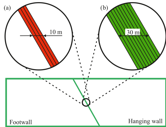
Figure 9. Sketch visualizing the representation of the fault zone by elastically weak 3-D elements with a thickness of (a) 10 m made from three elements or (b) 30 m made of nine elements. The elements outside this fault zone are not visualized.
