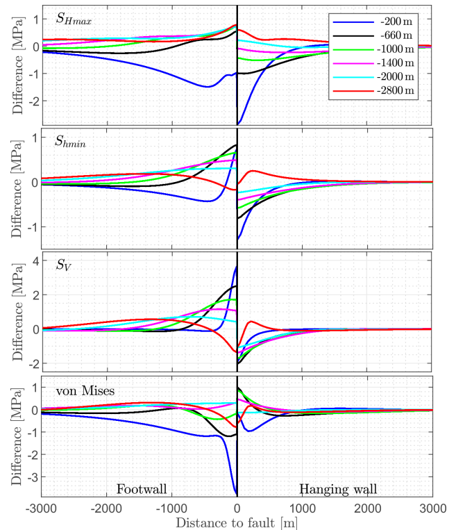
Figure 7. Variations of the stress components ( S_{Hmax} , S_{hmin} , S_V , and von Mises stress) at different depth levels are shown with respect to the distance of the fault. Stress magnitude changes are visualized along a vertical line at depths of -200 , -660 (reference depth, used by the other figures), -1000 , -1400 , -1400 , -2000 , and -2800 m.
