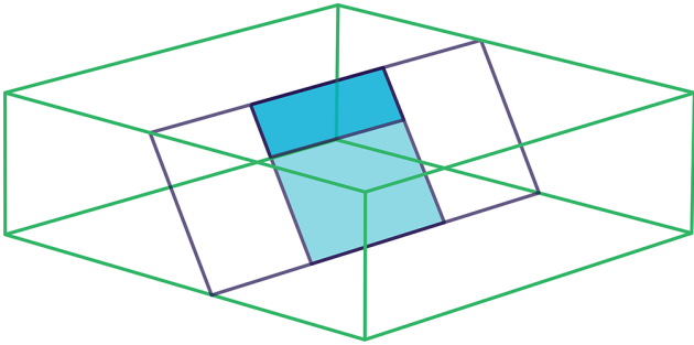
Figure 21. Model sketch with a reduced fault surface area of 4 \times 3 \text{ km}^2 (light and dark blue areas together) and 4 \times 1 \text{ km}^2 size (dark blue area only). Everything else is the same as shown by Fig. 3.
