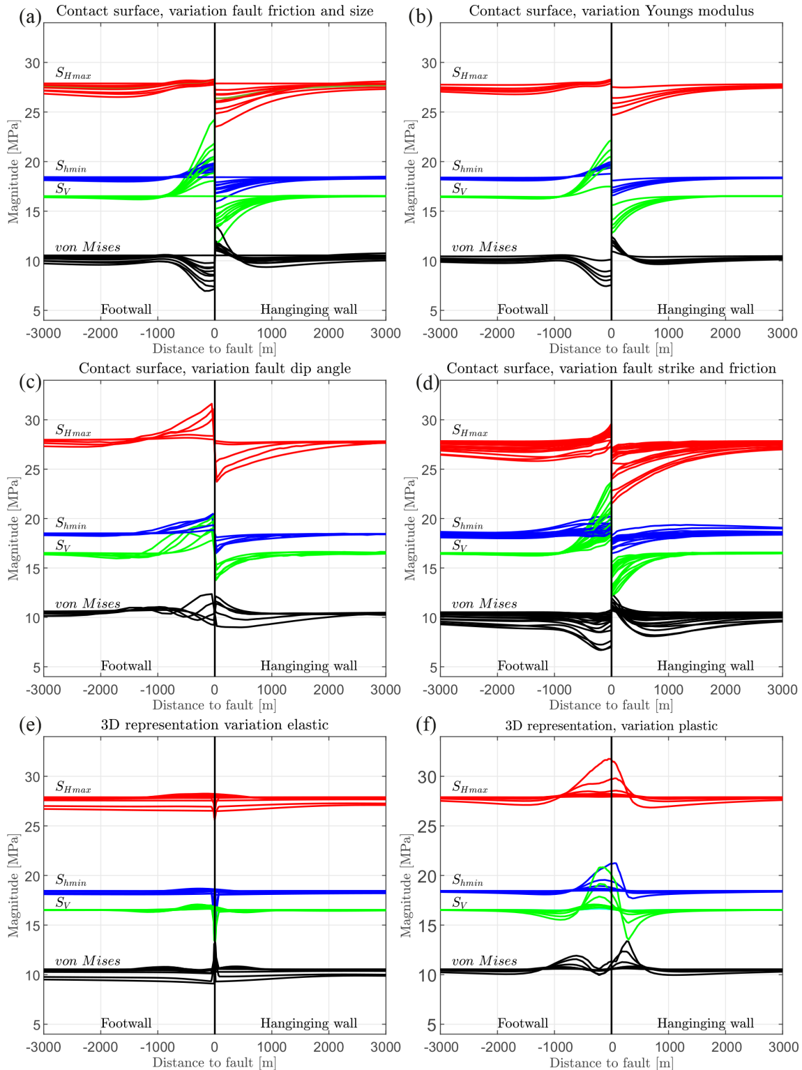
Figure 24. Summary illustration of the results from various presented models. Panel (a) shows the impact of the fault friction ( \mu = 0.1, 0.2, 0.4, 0.6, 1.0 , and > 1.0 ) using contact elements (Fig. 8) and the influence of the fault size and model size (Fig. 22). Panel (b) displays the influence of a variable Young's modulus of the host rock on the stress state near the fault and far from the fault (Fig. 20). Panel (c) shows the impact of a variable fault dip (Figs. 15 and 16), where (d) illustrates the impact of a variable fault strike and additionally friction variation ( \mu = 0.1, 0.2, 0.3 , and 0.4 ) on the stress state resulting from a fault represented by a contact surface (Figs. 17 and 18). The impact of a fault representation by 3-D elements is shown, where (e) elastically weak elements have a different stiffness (Figs. 10 and 11) and (f) where the elements are allowed to plastify as a result of a variable low friction (Fig. 14) and a laterally variable number of elements (Fig. 13).
