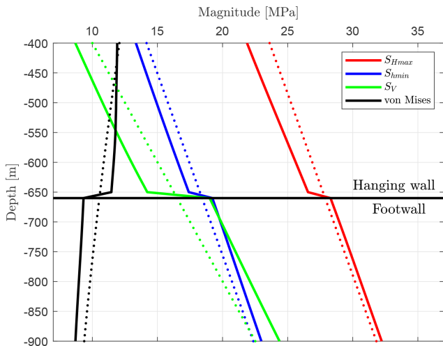
Figure 25. Stress magnitudes from a virtual well section for the depth range of -400 to -900 m of the reference model having contact surfaces (continuous line) and a model without a fault (dotted line).
