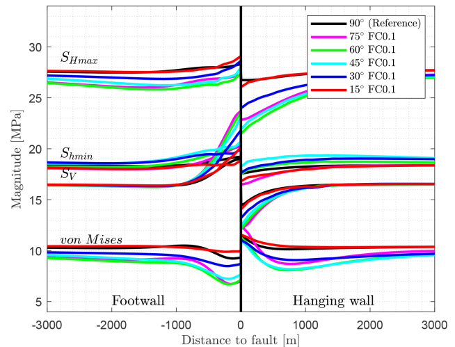
Figure 18. Variation of the strike angle, with 90 (reference), 75, 60, 45, 30, and 15^\circ relative to the orientation of the direction of maximum shortening. A friction coefficient of \mu = 0.1 is used in contrast to the similar models with a friction coefficient of \mu = 0.4 (Fig. 17). The stress components are plotted perpendicular to the strike of the fault.
