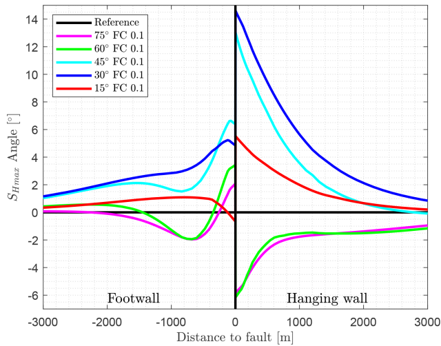
Figure 19. Variation of the strike angle (75, 60, 45, 30, and 15°) relative to the orientation of the maximum shortening direction using a friction coefficient of 0.1. Shown are the variations of the S_{Hmax} orientation compared to the reference model with a fault strike angle of 90° and a constant S_{Hmax} orientation of 0°. The angular variation is plotted perpendicular to the strike of the fault.
