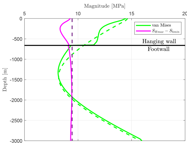
Figure 26. The von Mises stress and the difference between the two horizontal stresses ( S_{Hmax} - S_{hmin} ) are shown for the reference model with contact surfaces (continuous line) and a model with a continuous mesh (dotted line).
