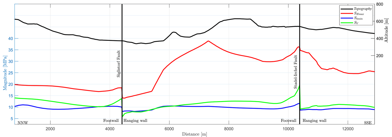
Figure 2. Plot of stress components along a NNW–SSE profile at approximately 400 m depth (sea level) within the Nördlich Lägern model (Hergert et al., 2015). The largest and smallest horizontal principal stress ( S_{Hmax} and S_{Hmin} ) as well as the vertical stress ( S_V ) are shown. Additionally shown is the topography from the model. The locations of the implemented Siglistorf and Stadel–Irchel faults are indicated by vertical black lines. Stress magnitude changes are significant next to the faults, but stresses are also variable due to a variable topography, rock stiffness, or other factors. The significant variation in S_{Hmax} is attributed to material changes, as the stratigraphic boundaries dip slightly towards the south.
