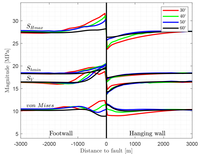
Figure 16. Influence of the fault dip angle on the stress components. A range of fault dip angles is presented, including 60 (reference model), 50, 40, and 30^\circ . By reducing the dip angle, the stress magnitude changes and the distance of the lateral stress perturbation increases. The most pronounced stress perturbation is seen for shallow dipping faults ( 30^\circ in red).
