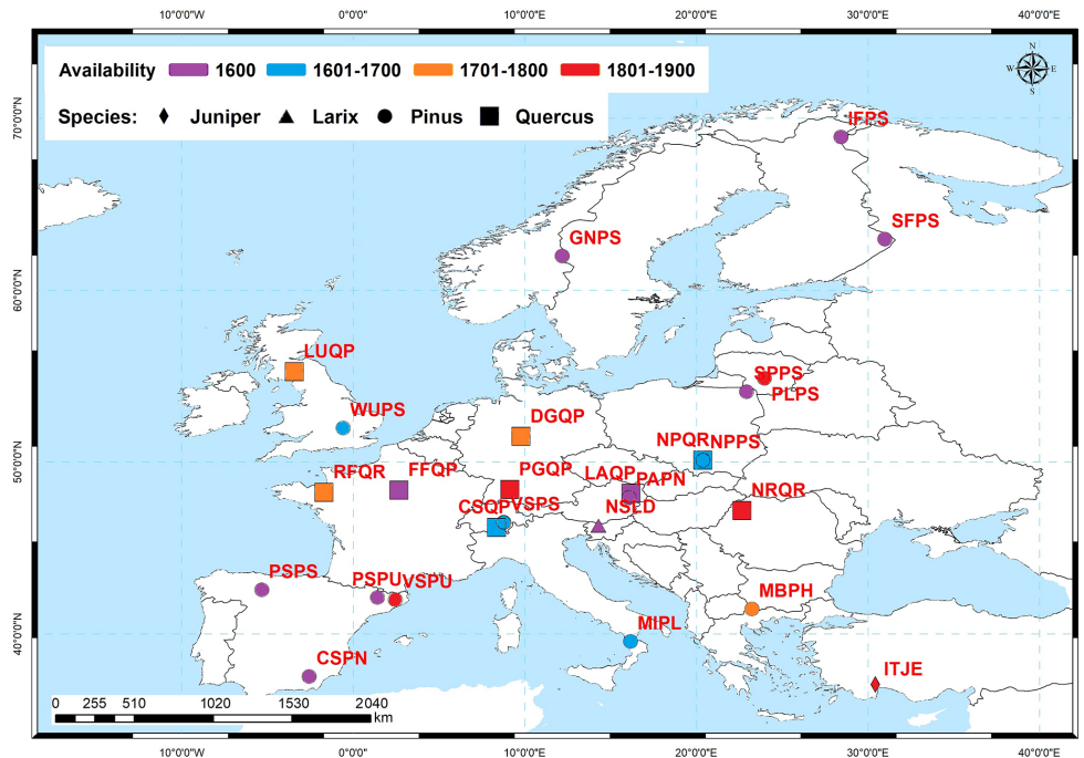
Figure 1. The site distribution of the \delta^{18}\text{O} network composed of 21 ISONET and 5 additional datasets (see Table 1). Colors indicate the past temporal availability of each tree ring dataset: starts in 1600 or earlier (purple), starts between 1601 and 1700 (blue), starts between 1701 and 1800 (orange), and starts between 1801 and 1900 (red). Symbols indicate tree species used for each record: Juniper (diamond), Larix (triangle), Pinus (circle), and Quercus (square).
