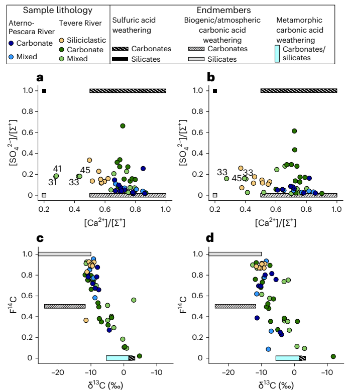
Fig. 2 | Water chemistry in relation to the expected chemical signatures of critical-zone weathering and metamorphic carbon. a, b , Ratios of [\text{Ca}^{2+}]/[\Sigma^+] plotted against ratios of [\text{SO}_4^{2-}]/[\Sigma^+] for winter samples ( a ) and summer samples ( b ). c, d , \delta^{13}\text{C} plotted against F^{14}\text{C} for winter samples ( c ) and summer samples ( d ). Samples are coloured by the dominant lithology in the upstream area 21 : carbonate, mixed carbonate and siliciclastic, or siliciclastic. Bars represent ion or isotopic endmember compositions 21 . Annotated samples in a and b are samples with low [\text{Ca}^{2+}]/[\Sigma^+] that have higher [\text{Na}^+] than [\text{Ca}^{2+}] and reflect evaporite \delta^{34}\text{S} and \delta^{18}\text{O}(\text{SO}_4) signatures.
