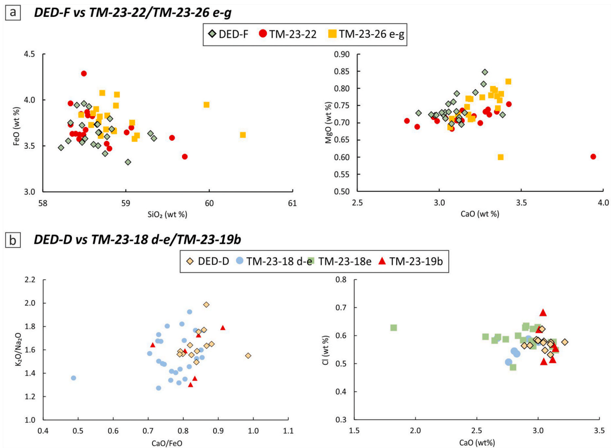
Fig. 7. Comparison between the investigated DED-F and DED-D and their equivalents. a) Major element composition of DED-F in comparison with the Monticchio tephtras TM-23-22/TM-23-26-e-g (Wulf et al., 2004). b) Major element composition of DED-D in comparison with the Monticchio TM-23-18-d-e/TM-23-19b (Wulf et al., 2004).
