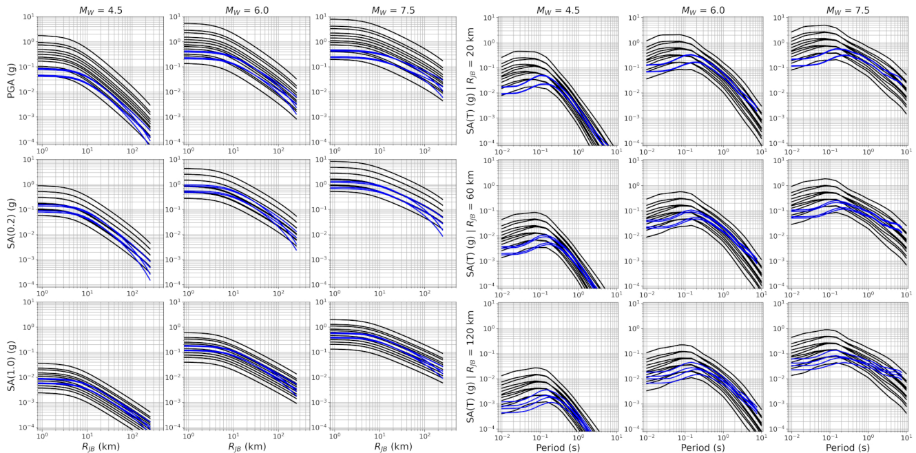
Figure 7. As Fig. 3 but for the craton scaled-backbone GMM logic tree. Expected ground motions corresponding to the parametric craton model (Eq. 5) are shown in black, while the selected branches of the default shallow-seismicity model are in blue.
