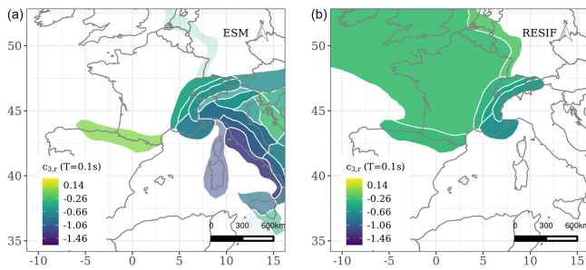
Figure 8. Distributions of \delta_{c3,R} for T \approx 0.1 s calibrated according to the ESM database (a) and the Résif database (b). Figure adapted from Kotha (2020).
