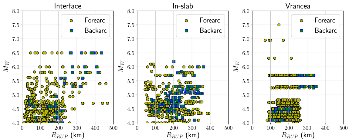
Figure 15. Magnitude and distance distributions of the selected records classified according to interface, as in-slab and for the Vrancea deep seismic zone.
