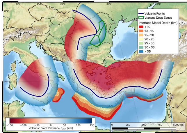
Figure 21. Definition of the subduction interfaces, the volcanic fronts (dark blue lines), and Vrancea deep source zones (green), along with variation in R_{XVF} used for ESHM20. Backarc regions are shown in red and forearc regions in blue. Figure adapted from Danciu et al. (2021).
