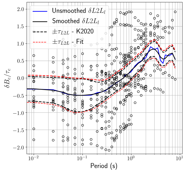
Figure 12. Distribution of between-event residuals with period for the Iceland ground motion data, with fit models of \delta L2L_l(T) and its variability \tau_{L2L} .
