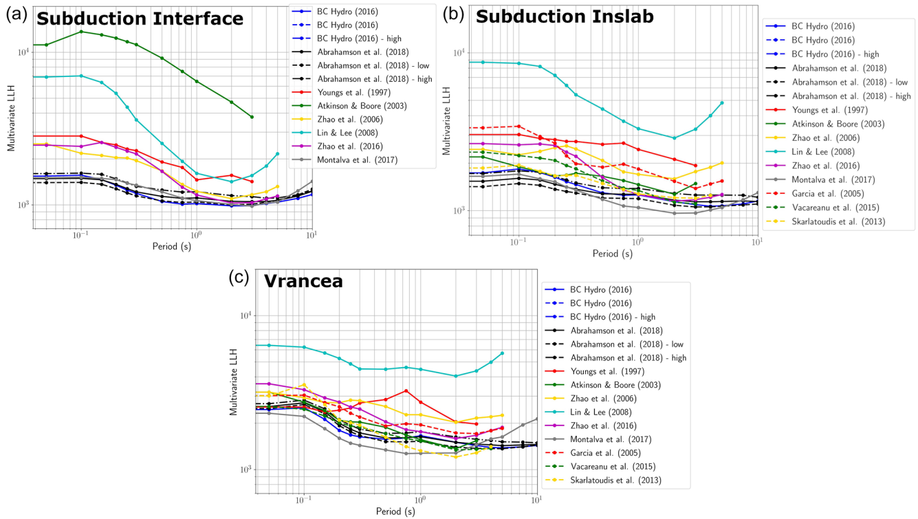
Figure 16. Variation in multivariate log-likelihood ( \ell\ell ) with period for each GMM considered for the subduction interface (a), subduction in-slab (b) and Vrancea (c) regions.
