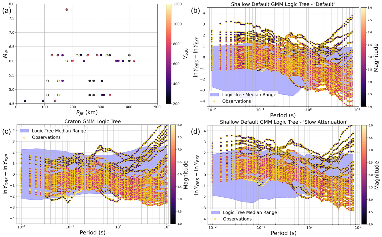
Figure 10. Magnitude and distance distribution of Portuguese records from RESORCE used for the analysis (a) and comparison of the distribution with the period of residuals of observed ground motions with respect to the backbone GMM for the default shallow GMM logic tree (b), the craton GMM logic tree (c) and the slow-attenuation cluster GMM logic tree (d). The shaded regions describe the range of expected ground motions from the logic tree across all the considered scenarios, centred such that 0 describes the unadjusted backbone GMM for each logic tree. Points corresponding to \ln(Y_{OBS}) - \ln(Y_{EXP}) are colour scales according to the earthquake magnitude.
