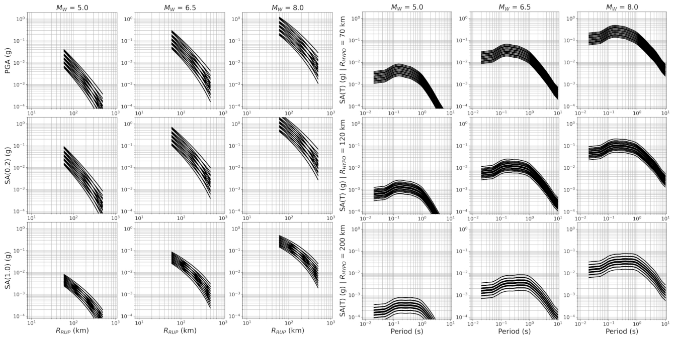
Figure 20. As Fig. 19 but for the subduction in-slab and Vrancea deep zone scaled-backbone GMM logic tree. Magnitudes considered at M_W 5.0, 6.5 and 8.0 (columns) and distances R_{HYPO} = 70, 120 and 200 km respectively. Sites are assumed to be forearc with V_{S30} 800 \text{ m s}^{-1} .
