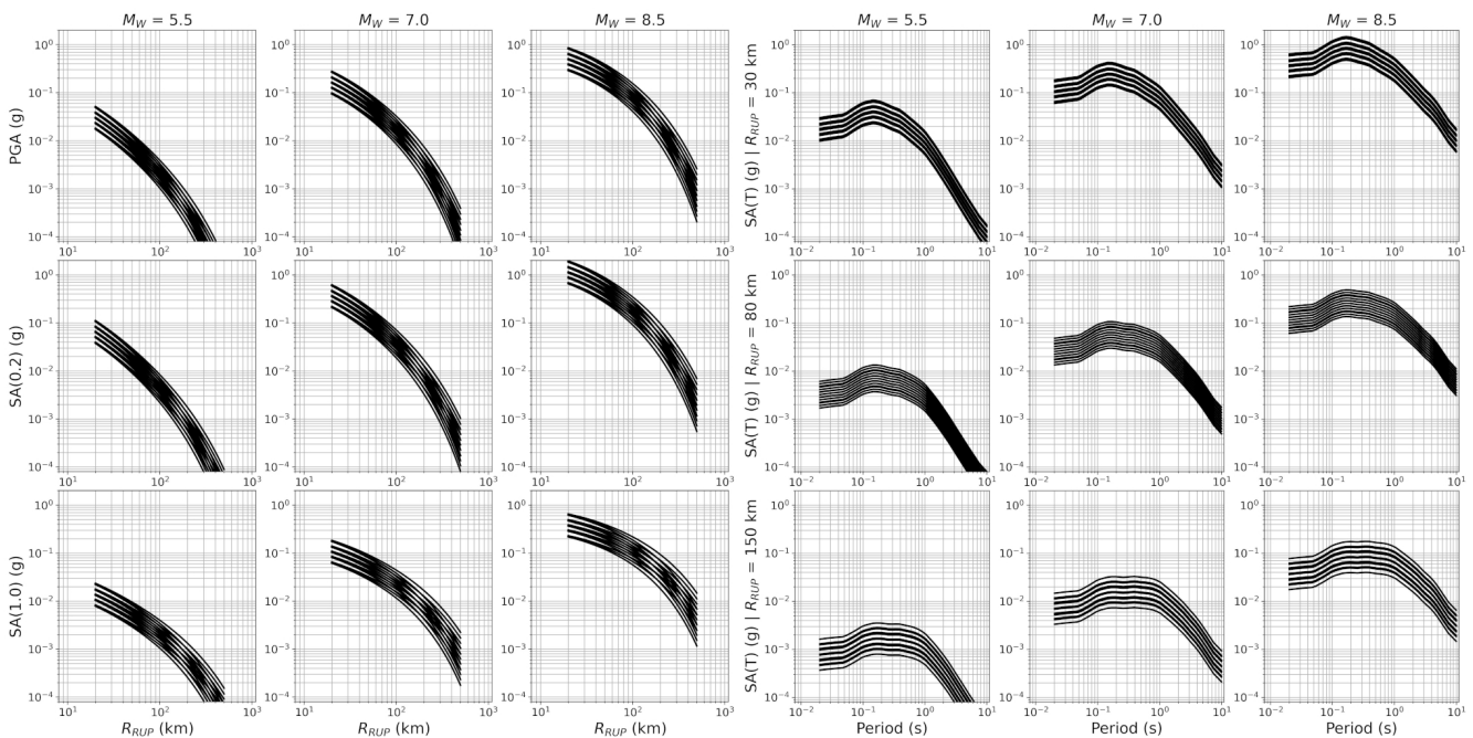
Figure 19. As Figs. 3 and 7 for the subduction interface scaled-backbone GMM logic tree. Magnitudes considered at M_W 5.5, 7.0 and 8.5 (columns) and distances R_{RUP} = 30, 80 and 150 km respectively. Sites are assumed to be forearc with V_{S30} 800 \text{ m s}^{-1} .
