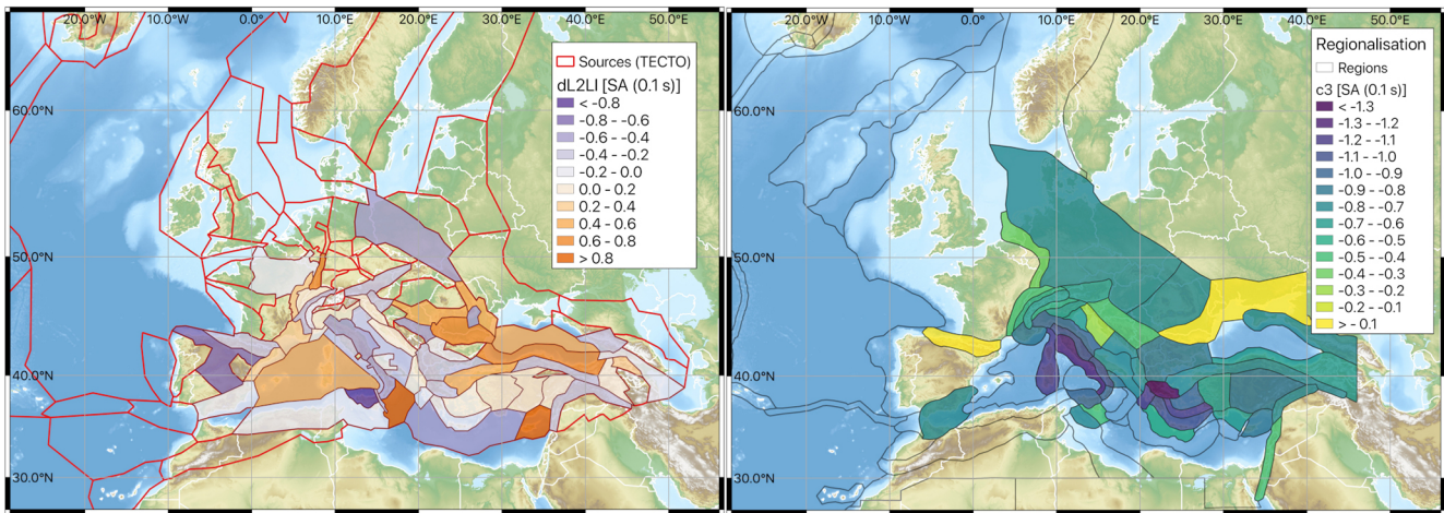
Figure 2. Regional variation in \delta L2L_l (left) and c_3 + \delta c_{3,r} (right) for Sa (0.1 s) using the TECTO and Basili et al. (2021) regionalisations respectively (Figures reproduced from Weatherill et al., 2020).
