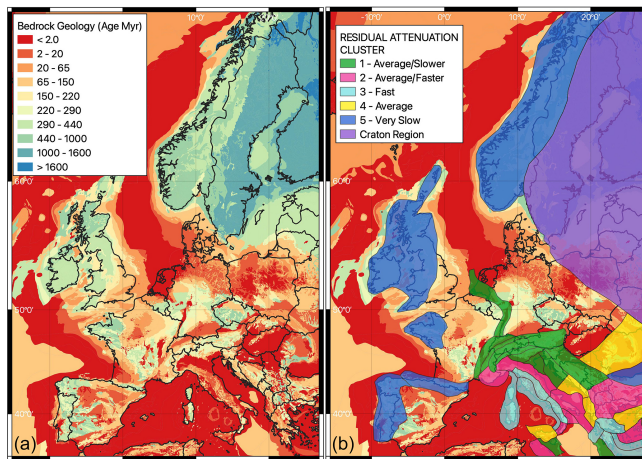
Figure 9. Bedrock geology across Europe from the 1 : 5 000 000 International Geological Map of Europe (Asch, 2005) coloured according to age (a) and updated regionalisation depicting the final spatial extent of the slow-attenuation cluster (b).
