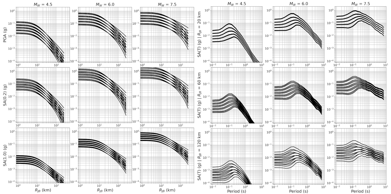
Figure 3. Expected ground motion from all 15 branches of the default backbone GMM logic tree for shallow seismicity shown in terms of attenuation with distance (left image) and scaling with spectral period (right image). Columns refer to M_W 4.5, 6.0 and 7.5 respectively, while rows refer to intensity measures PGA, Sa (0.2 s) and Sa (1.0 s) for attenuation, or to distances of R_{JB} 20, 60 or 120 km for Sa ( T ).
