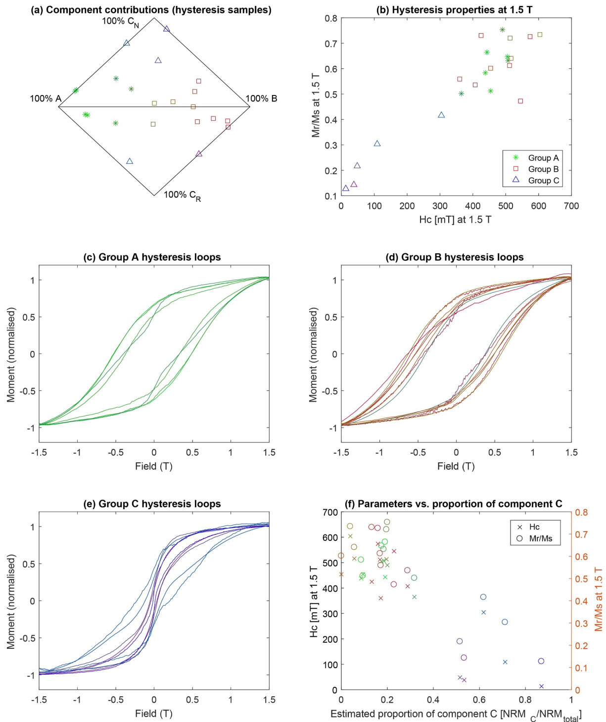
Figure 9. High field experiments. (a) Vector unmixing results for samples used in the hysteresis experiments, with dominant components indicated by blue triangles (C), red squares (B) and green stars (A). The same color shading is preserved in panels b–f. (b) Samples with higher M_r/M_s ratios have higher coercive forces ( H_c ). Lower H_c values can indicate larger hematite grain sizes (Özdemir & Dunlop, 2014), and/or mixtures of magnetite with hematite. (c–e) Room temperature hysteresis curves for specimens from component groups A, B, and C. Groups A and B have wide curves consistent with single domain hematite. Group C has wasp-waisted loops, indicating populations of grains with distinctly different coercivity spectra. (f) M_r/M_s and H_c values (at 1.5 T) correlate negatively with the proportion of component C.
