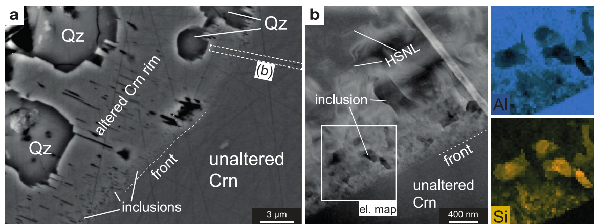
Fig. 7 Investigations on the Si reaction rim in natural Crn from Setup 5 (run 29). a The altered Crn rim (see Figure 6b for overview) shows an accumulation of nanometer sized inclusions along reaction front (or at the contact with unaltered Crn, marked with dashed white line; BSE image). Numerous larger Qz grains are located inside the rim. b TEM investigations along the contact between reaction front and
