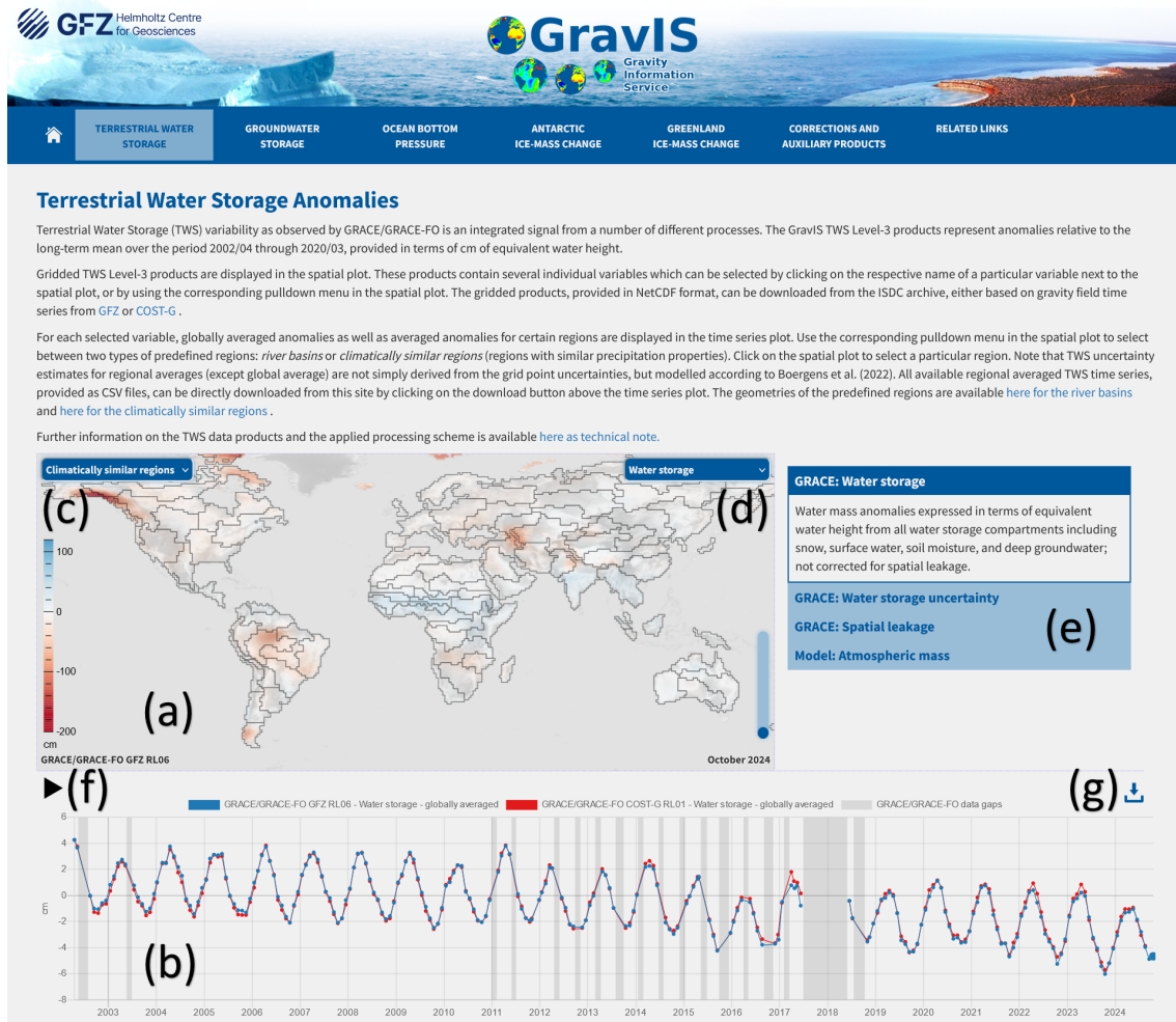
Figure 7. Screenshot of the GravIS subpage for TWS showing the following features: (a) zoomable map, (b) time series plot, (c) drop-down menu for selection of predefined regions, (d) drop-down menu for selection of product variables, (e) accordion menu with descriptions of product variables, (f) play/stop button for time series animation, and (g) download button for regional average products.
