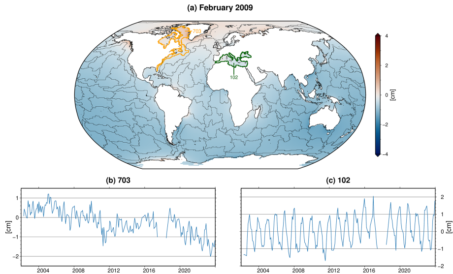
Figure 6. (a) Barystatic sea-level anomalies from the gridded GravIS Level-3 OBP product based on GFZ for February 2009. (b) Regionally averaged barystatic sea-level anomaly time series from 2002 to 2023 for the region along the eastern coast of North America, Hudson Bay, and Baffin Bay (marked with an orange boundary in panel a). (c) Same as (b) but for the region including the Mediterranean Sea and the Black Sea (marked with a green boundary in panel a). Visualization of all other product variables, including uncertainties and leakage, is available through the GravIS web portal ( https://gravis.gfz.de , last access: 21 January 2025).
