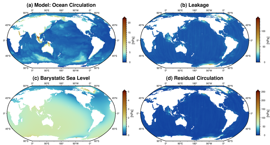
Figure 8. Temporal rms values (2002–2021) of ocean mass anomalies for different variables of the gridded GravIS Level-3 OBP product based on COST-G: (a) mean ocean circulation pressure from a background model (AOD1B); (b) apparent bottom pressure due to continental leakage; (c) barystatic sea-level pressure; (d) residual ocean circulation pressure.
