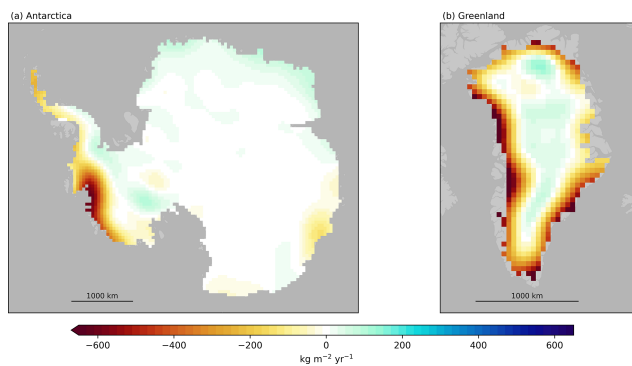
Figure 3. Spatial pattern of the linear mass change rate for the Antarctic (a) and Greenland (b) ice sheets from April 2002 to August 2023. The mass change rate is computed from the gridded GravIS Level-3 ice product based on COST-G.
