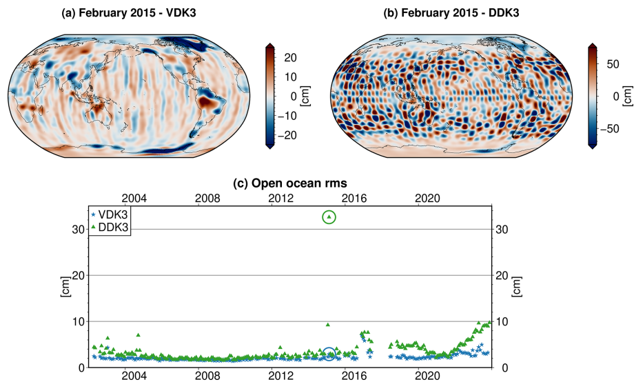
Figure 2. (a) GFZ RL06 Level-2 solution (max. SH degree 96) for February 2015 in terms of surface-mass densities [cm], filtered with VDK3. (b) Same as (a) but filtered with DDK3. (c) Open ocean rms values (distance to coast > 1000 km) for the GFZ GRACE/-FO RL06/RL06.1 time series when filtered with VDK3 (blue asterisks) and DDK3 (green triangles); values for February 2015 are circled.
