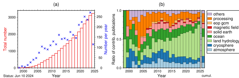
Figure 1. (a) Number of GRACE/-FO-related publications per year and their cumulative distribution. (b) Ratio of these publications contributing to predefined categories; in addition to the different Earth system compartments of atmosphere, cryosphere, land hydrology, ocean, and solid Earth, applications to the magnetic field, the Earth orientation parameters and geocentre motion (eop gcm), and data processing are distinguished. The considered database of GRACE/-FO-related publications is maintained at GFZ and currently contains 3228 peer-reviewed publications ( https://www.gfz.de/grace , last access: 10 June 2024).
