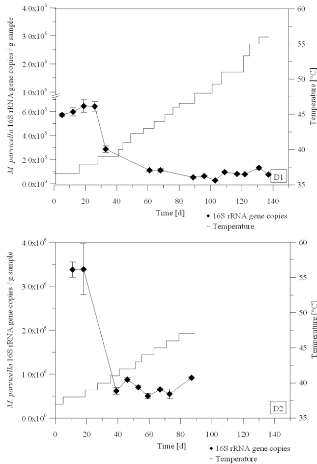
Figure 7: Quantification of M. parvicella in D1 and D2 in relation to the increase in temperature. 16S rRNA gene copy number per g of digestate decreased with increasing temperatures. In D1, a 6-fold decrease was detected at 43 °C. In D2, a decrease of about 10-fold was observed once the temperature was increased to 41 °C.
