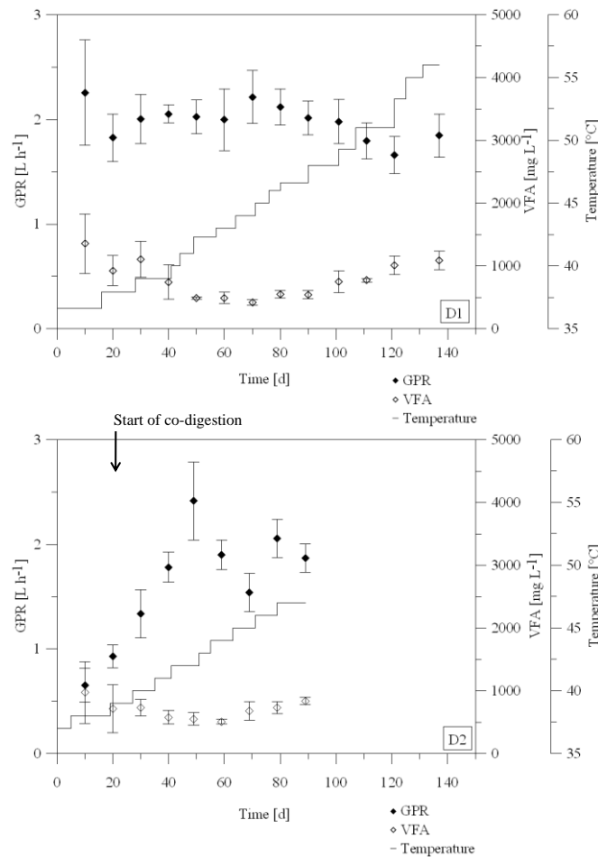
Figure 3: Volatile fatty acids (VFA) and gas production rate (GPR) in relation to the increase in temperature in digesters D1 and D2. Each data point represents the average of 10 days. GPR in D2 increased after daily oil addition from day 20 on.
