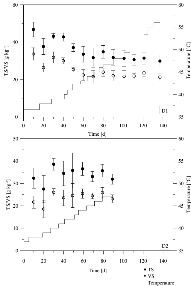
Figure 2: Total solids (TS) and volatile solids (VS) in relation to the temperature increase over time in digesters D1 and D2. Each data point represents the average of 10 days. Decrease in TS and VS values in relation to the increase in temperature during the first 60 days in D1 and constant values afterward. TS and VS values in D2 increased after daily oil addition from day 20 on.
