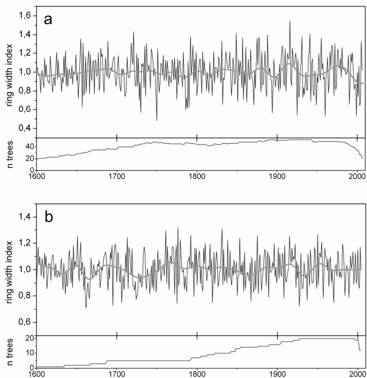
Figure 1: Residual ring-width chronologies (upper graphs) and their sample replication (lower graphs) for Juniperus polycarpus (a) and Quercus macranthera (b) in the northeastern Alborz Mountains, Iran. Bold curves indicate smoothed values by an 11-year FFT-filter.
