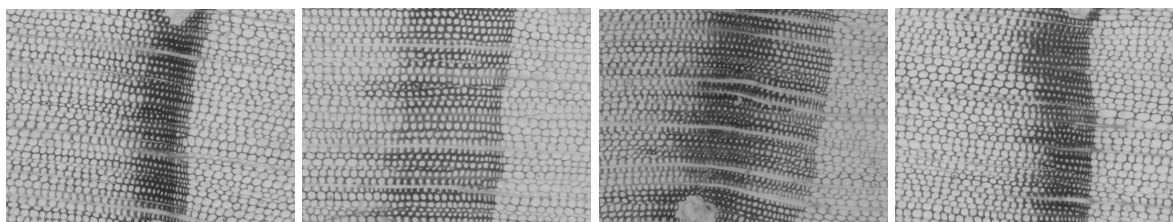
Figure 1: Examples of L+, 11, 211 and 12 rings.
