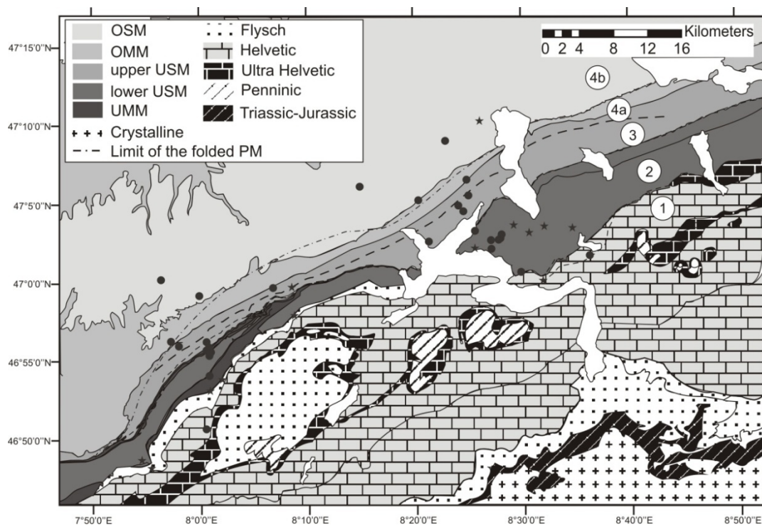
Figure 2-2: Detailed geological map of the study area with sample locations indicated. Black dots denote sampling localities for AFT and (U-Th-Sm)/He data analyzed by CvH, black stars denote sample points of AFT data analyzed by MR. Four tectonic slices (1-4) are indicated as discussed in the text. TS-4b represents the flat lying part of the Plateau Molasse.
