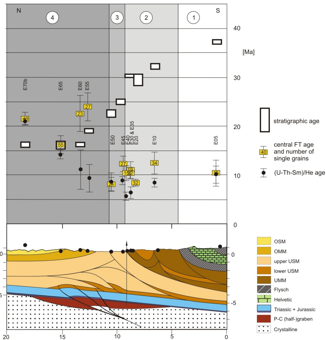
Figure 2-4: Profile across the Subalpine Molasse in the Entlebuch area, Switzerland. For location, see Figure 2-1. Black dots indicate the projected data points. The tectonic slices are taken from Figure 2-2. In the south, all thermochronology ages are significantly younger ages than the samples' stratigraphic ages, whereas in the north the opposite is true. Hence, an exposed palaeo-PAZ and PRZ lies in the tectonic slices south of TS-4.
