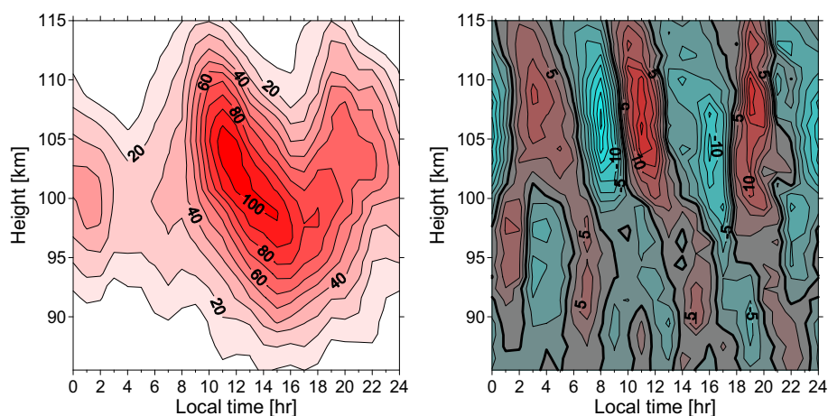
Figure 3 Example of occurrence frequencies (1/1,000) of sporadic E layers (left) and the corresponding residuals (right). The residuals are the occurrence frequencies after the mean, 12- and 24-h oscillations were subtracted. Shown are 3-monthly mean zonal means of October (September to November) 2010, covering the latitudes from 43° to 63° N.
