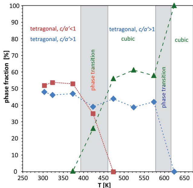
Fig. 5 The phase composition of the sample at a pressure of 1.87 GPa as a function of temperature obtained from the EDXRD experiment. Red squares: % of the tetragonal phase with c/a' < 1 ; blue diamonds: % of the tetragonal phase with c/a' > 1 ; green triangles: % of the cubic phase.
