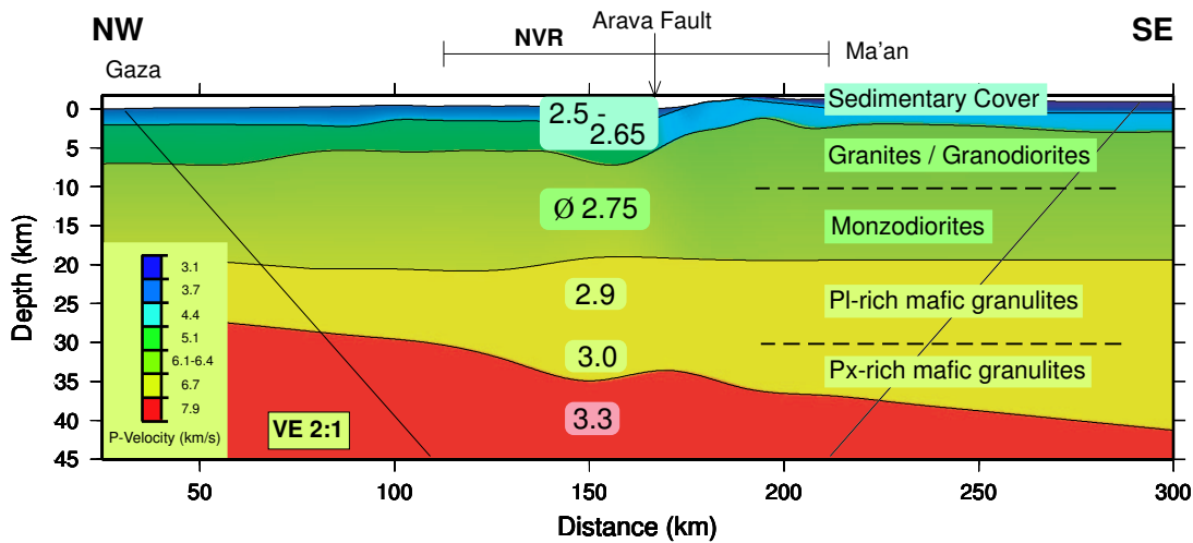
Figure 3.10: Crustal model along the WRR profile; the WRR P velocities are colour-coded (DESERT Group, 2004), the numbers represent density values in \text{g}/\text{cm}^3 from gravity modelling (El-Kelani et al. , 2003). The petrology is after H.-J. Förster (pers. comm., 2003)
