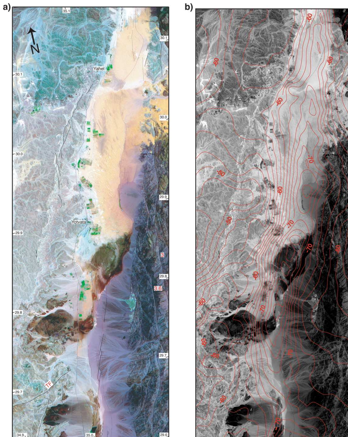
Figure 4.1: a) ASTER scene of the southern Arava Valley taken on June, 6th, 2000. The southern margin is located \sim 10 km north of the Gulf of Aqaba. Solid lines represent unambiguous faults; dashed lines are lineaments related to subsurface faults seen in seismic reflection data (Frieslander, 2000; Shtivelman et al. , 1998); dotted lines are lineaments of unknown origin. The red numbers represent the amount of sinistral strike-slip motion, that is observed at the faults to their left. TF: Themed Fault. b) Same area as shown in a) in red are contour lines (values in mGal) of a Bouguer gravity study by ten Brink et al. (1999).
