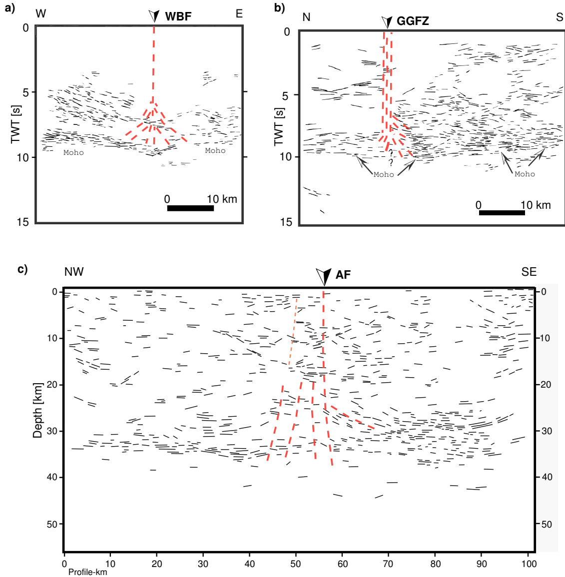
Figure 5.1: Comparison of two interpretive line drawings by Stern and McBride (1998) (a and b) to the NVR profile (c). Dashed red lines indicate the locus of deformation associated with strike-slip, not necessarily faults themselves. a) Interpretive line drawing of a time-migrated seismic reflection profile across the Walls Boundary Fault (WBF), the northern continuation of the Great Glen Fault north of the Shetland Islands, based on a section from McBride (1994); b) Interpretive line drawing of a profile across the Great Glen Fault Zone (GGFZ) north of northern Ireland, based on a frequency-wavenumber migration by Klemperer et al. (1991); c) Manual interpretive line drawing of the DESERT NVR profile. The thinner dashed line west of the Arava Fault (AF) indicates the existence of an older, inactive fault segment.
