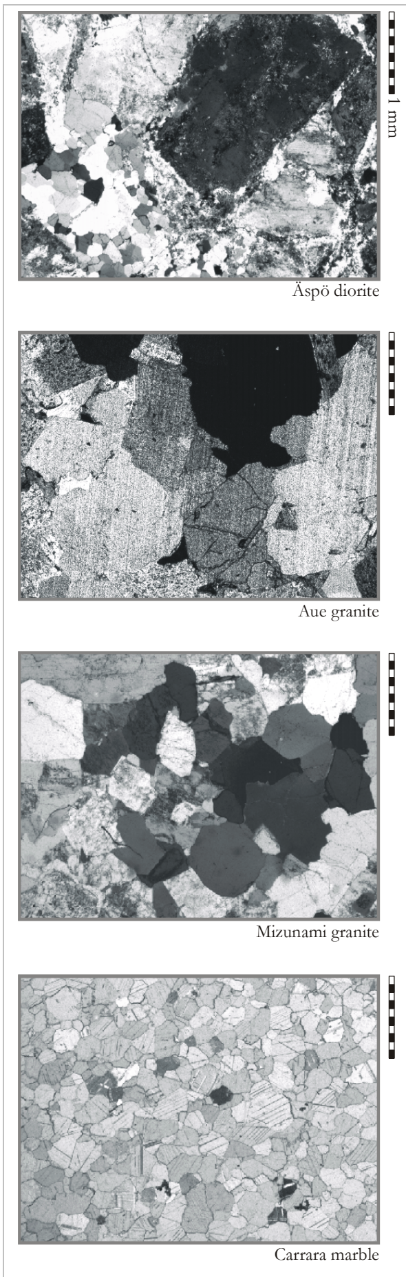
Fig. 3-3. Micrographs of undeformed samples of each rock type taken with crossed nicols. All micrographs are the same scale.
