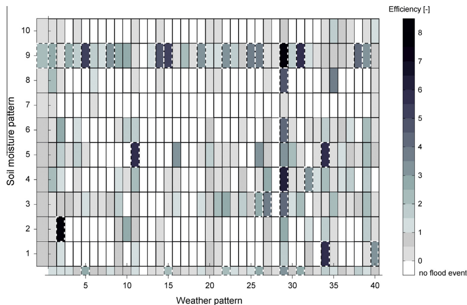
Fig. 7. Efficiencies of soil moisture and weather patterns respectively (margins) as well as efficiencies of soil moisture-weather pattern combinations (matrix). Soil moisture patterns are considered at the event start date. The weather patterns are considered in the event build-up period. Dashed framed panels show a significant flood-prone relationship.
