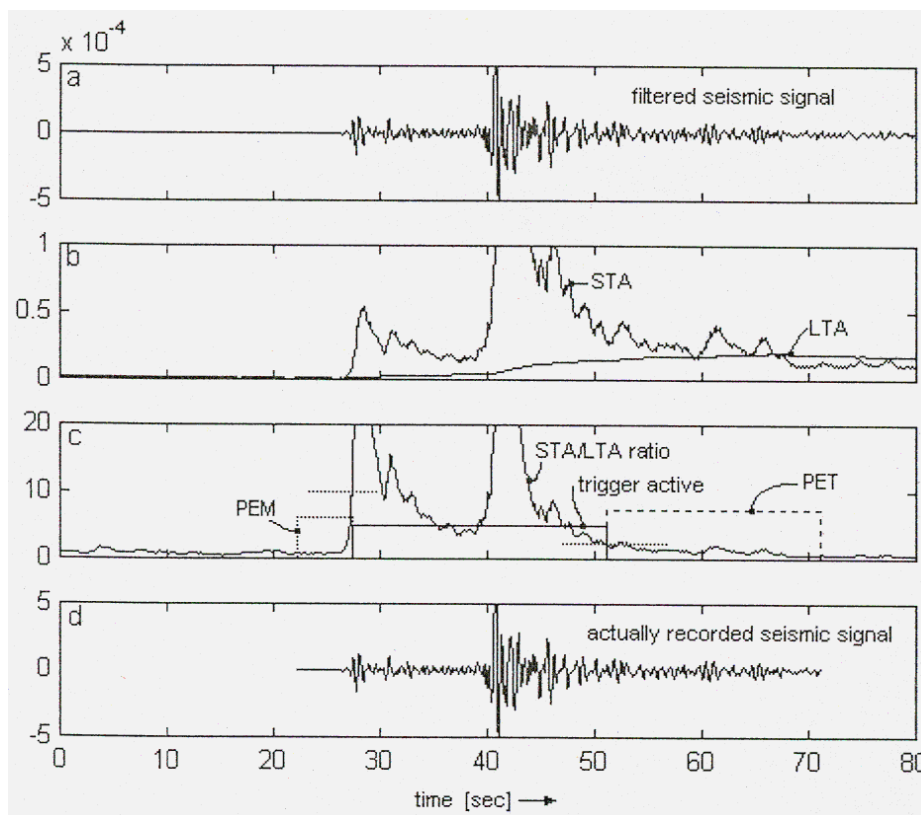
Figure 1 Function and variables of STA/LTA trigger calculations (see text for explanations).
